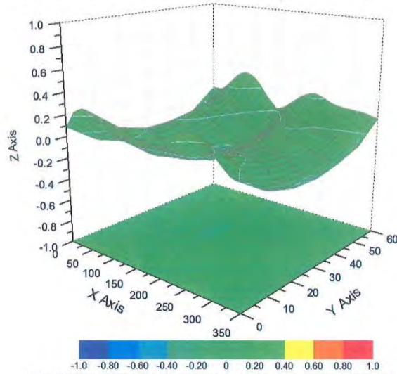
Uncertainty of Spherical Isotropy Assessment: \pm 3.2\% (K=2)
