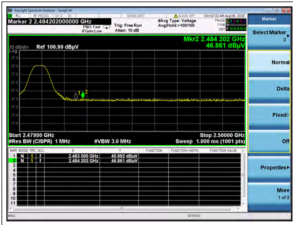
(PEAK, Channel 39)
