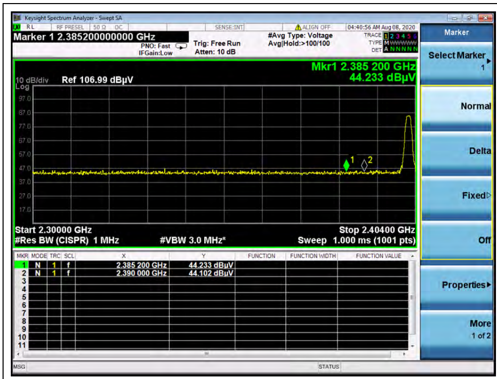
(AVERAGE, Channel 0)
