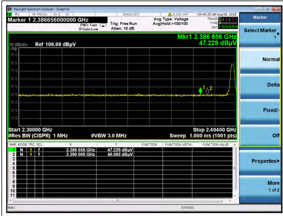
(PEAK, Channel 0)
