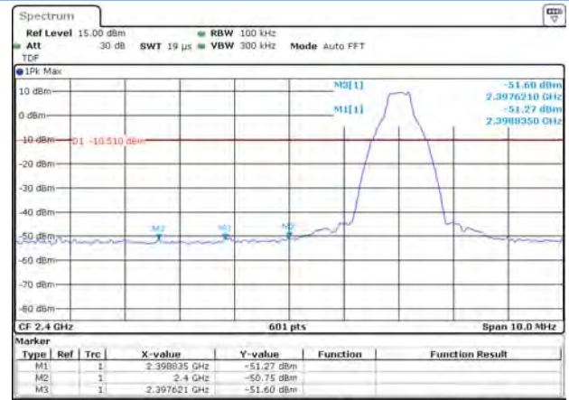
GFSK LOW CHANNEL, BAND EDGE
