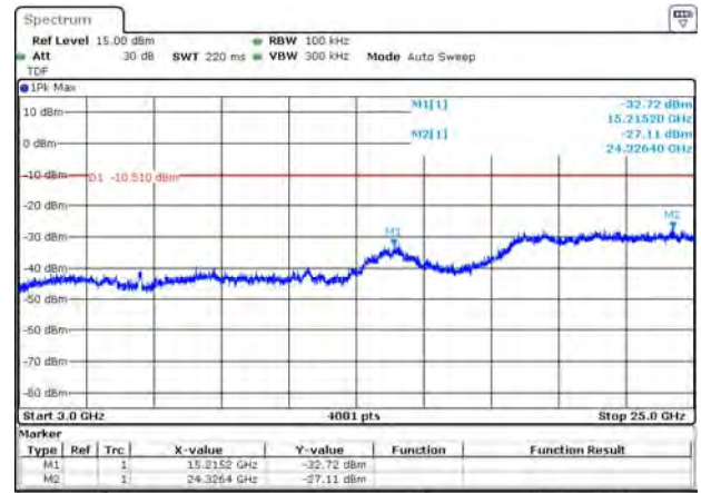
GFSK LOW CHANNEL, SPURIOUS 3 GHz ~ 25 GHz
