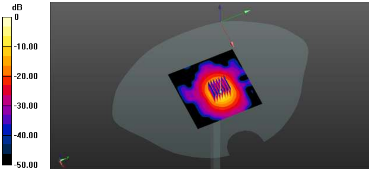
0 dB = 17.1 W/kg
