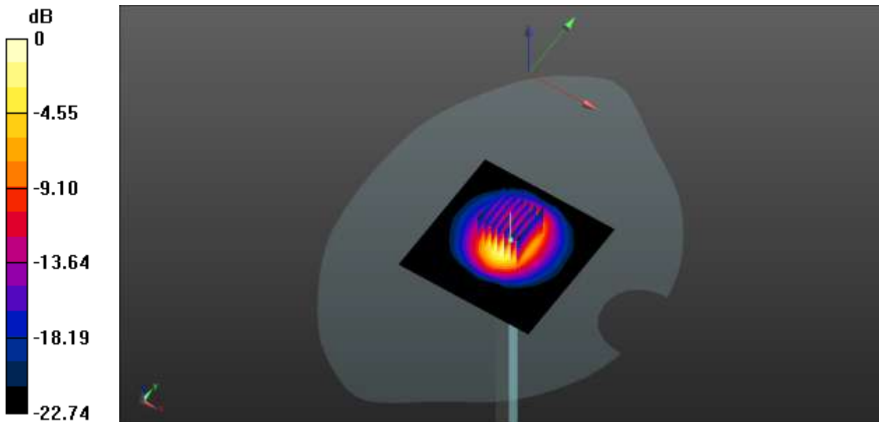
0 dB = 6.08 W/kg
