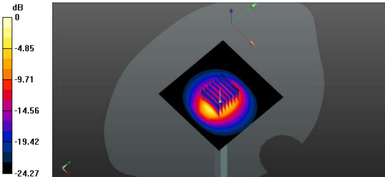
0 dB = 6.36 W/kg
