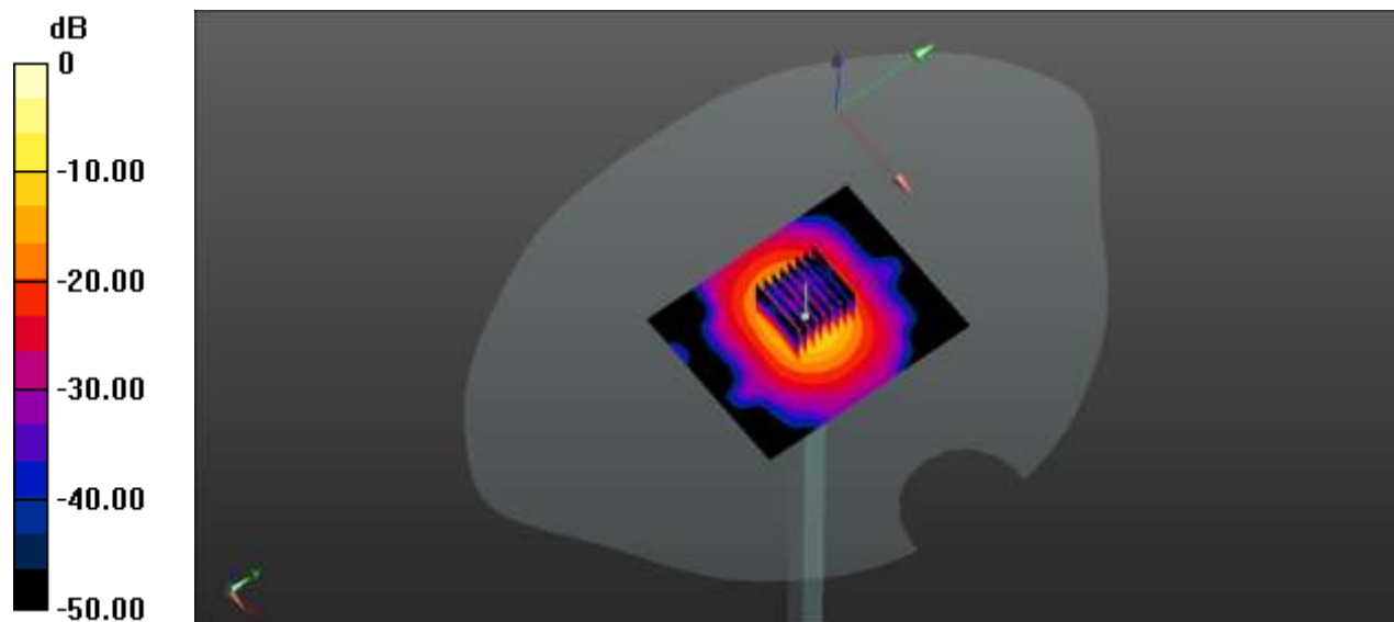
0 dB = 19.4 W/kg
