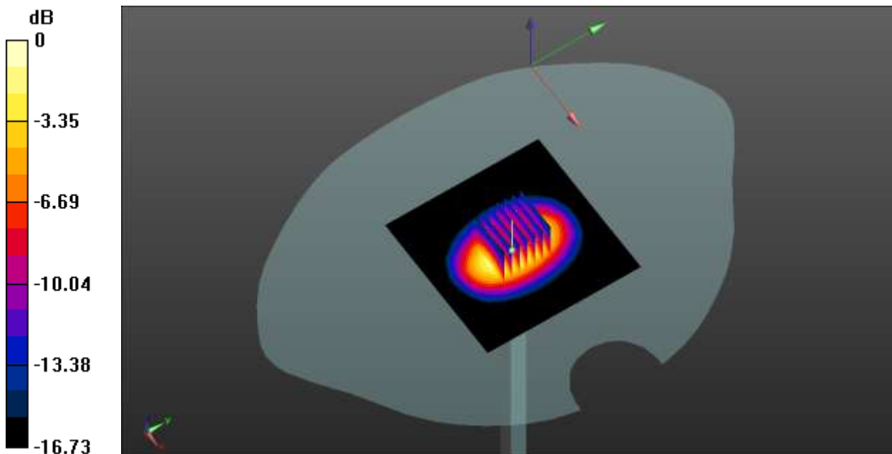
0 dB = 4.58 W/kg
