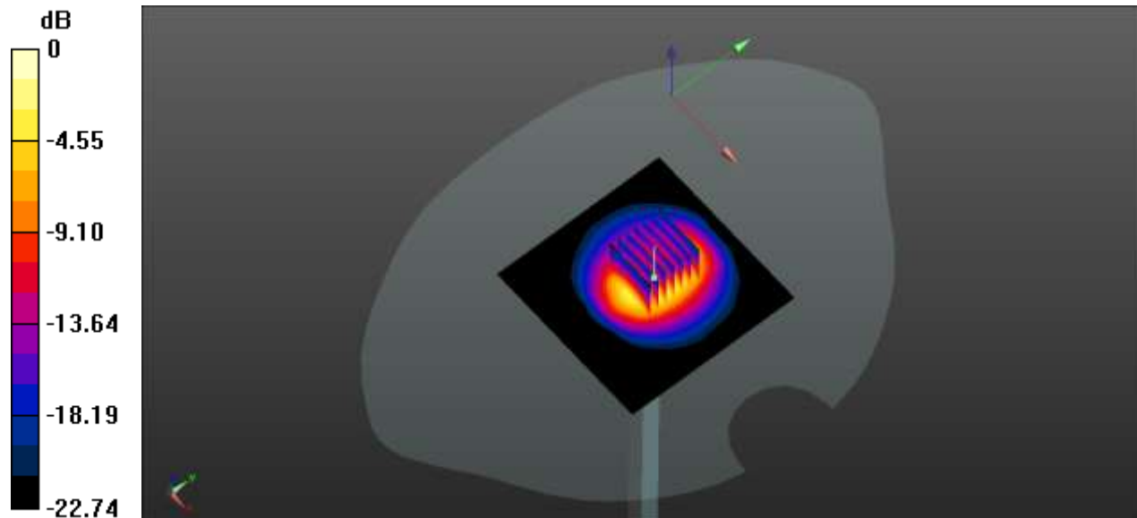
0 dB = 5.81 W/kg
