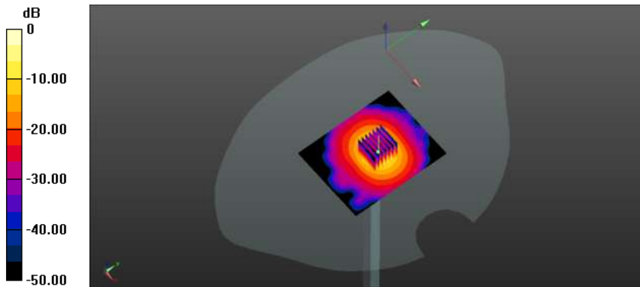
0 dB = 14.6 W/kg
