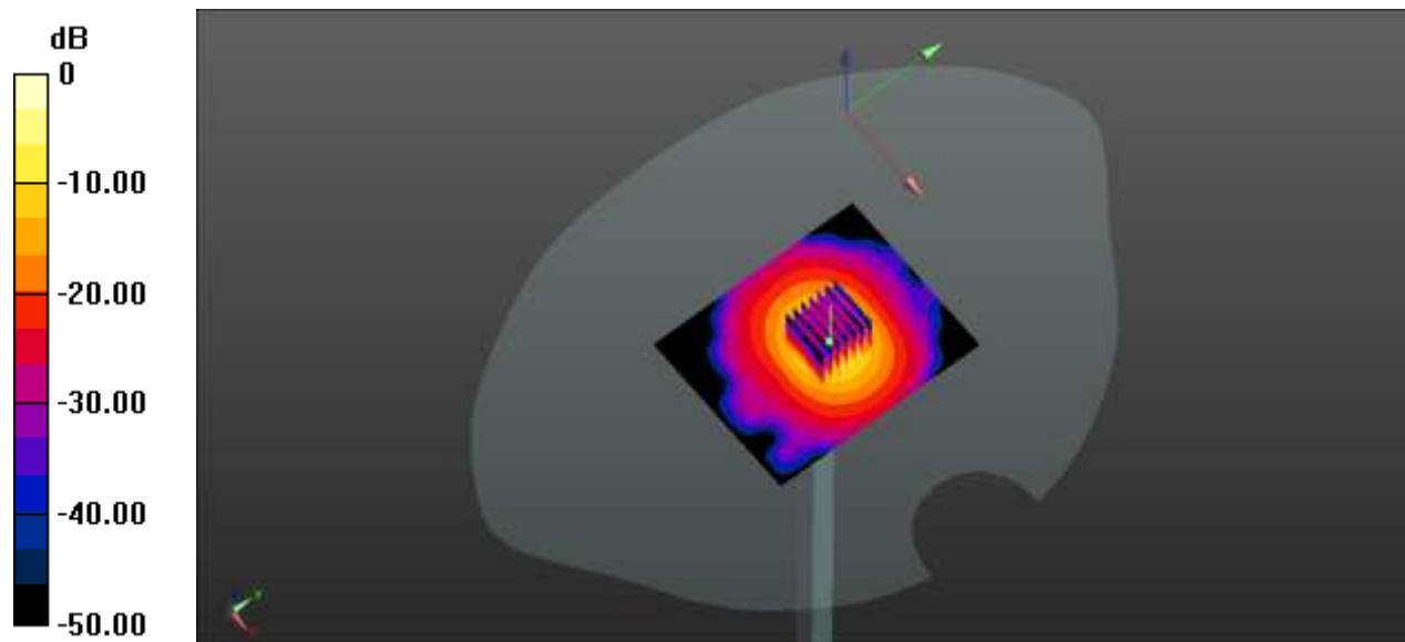
0 dB = 15.3 W/kg
