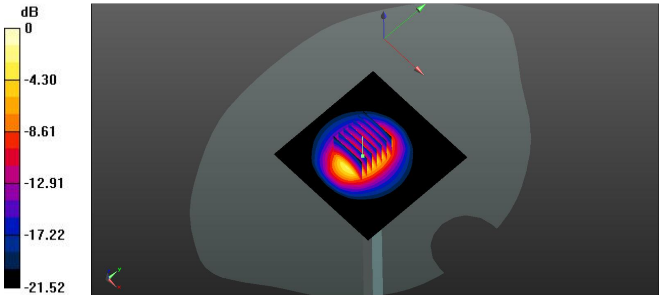
0 dB = 6.10 W/kg
