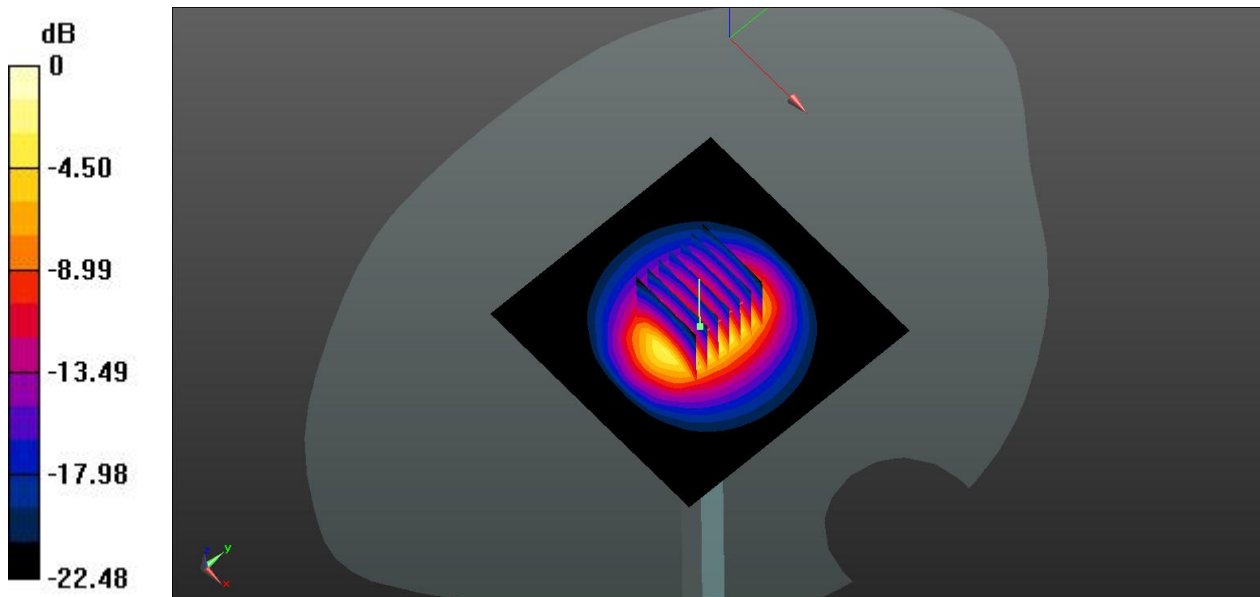
0 dB = 6.06 W/kg
