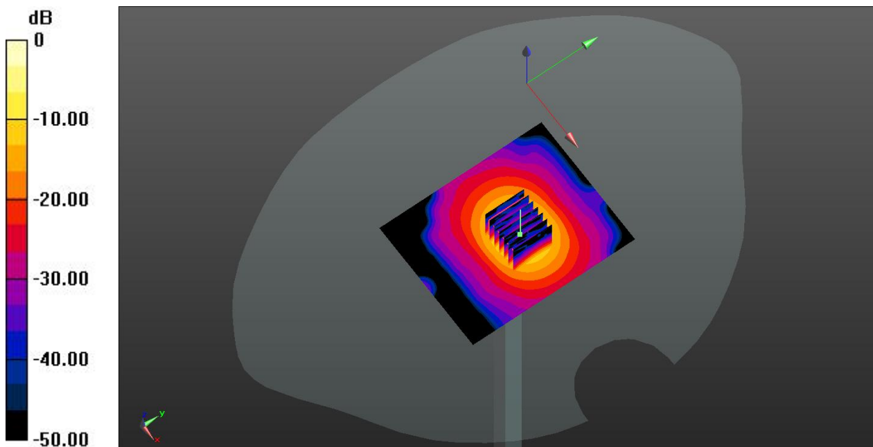
0 dB = 16.3 W/kg
