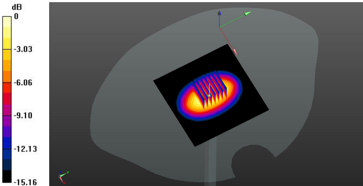
0 dB = 4.16 W/kg
