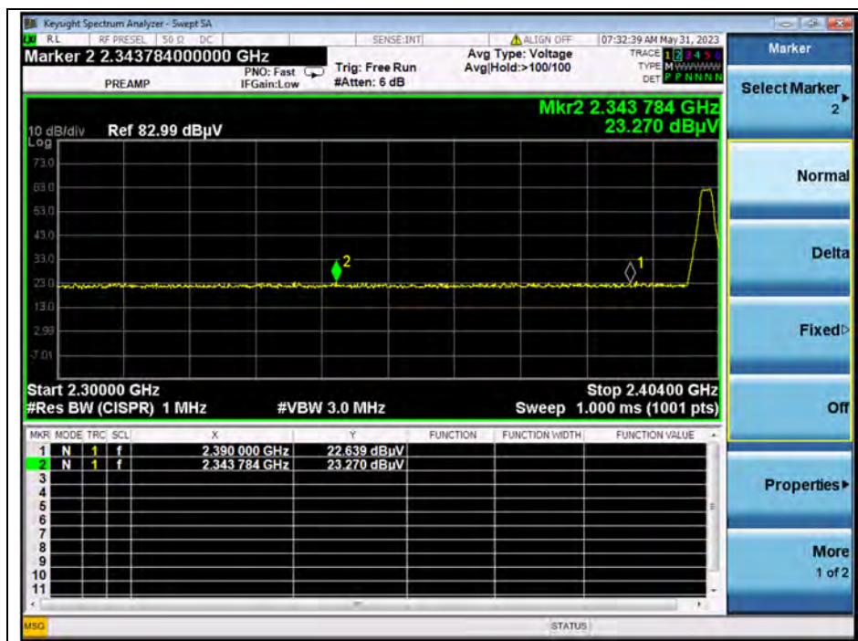
(PEAK, Channel 0)
