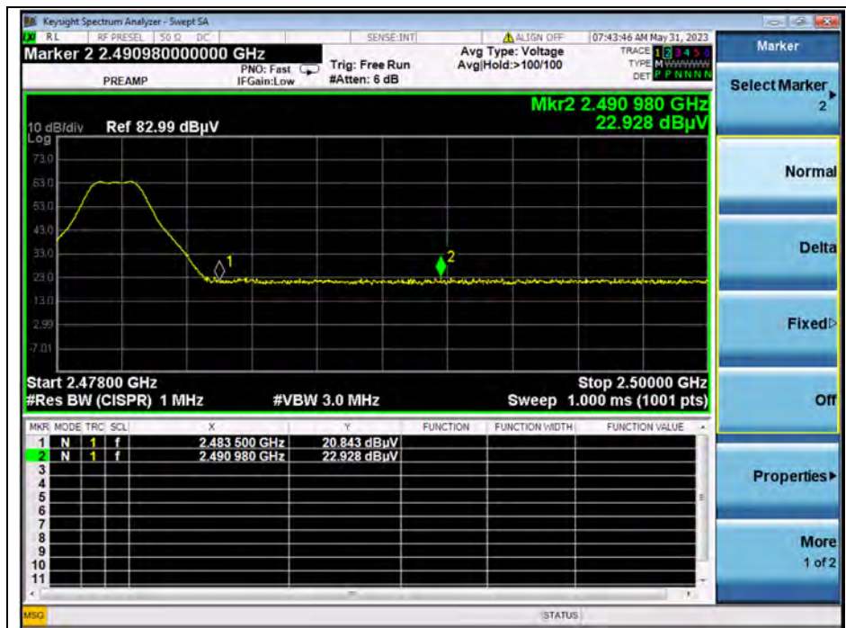
(PEAK, Channel 39)
