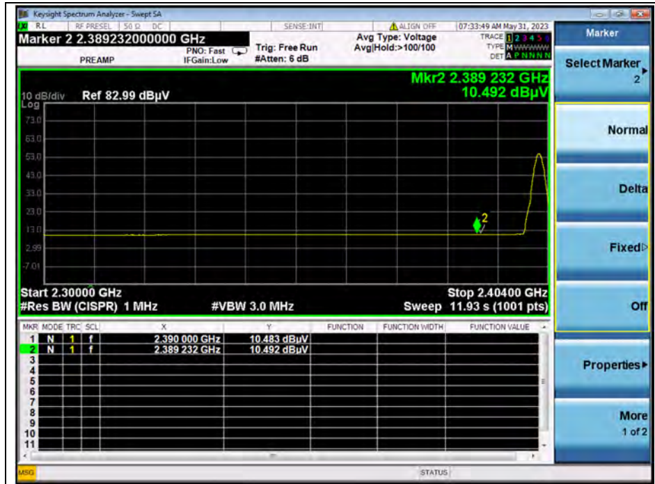
(AVERAGE, Channel 0)
