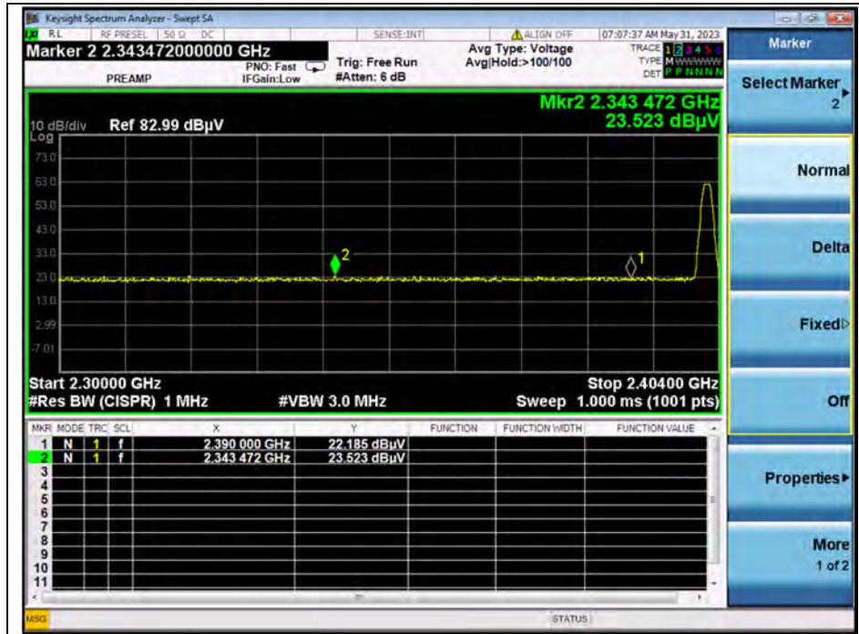
(PEAK, Channel 0)
