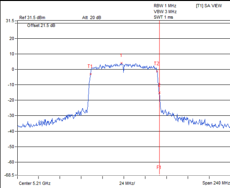
802.11ac(VHT80)_Chain0 / CH42
