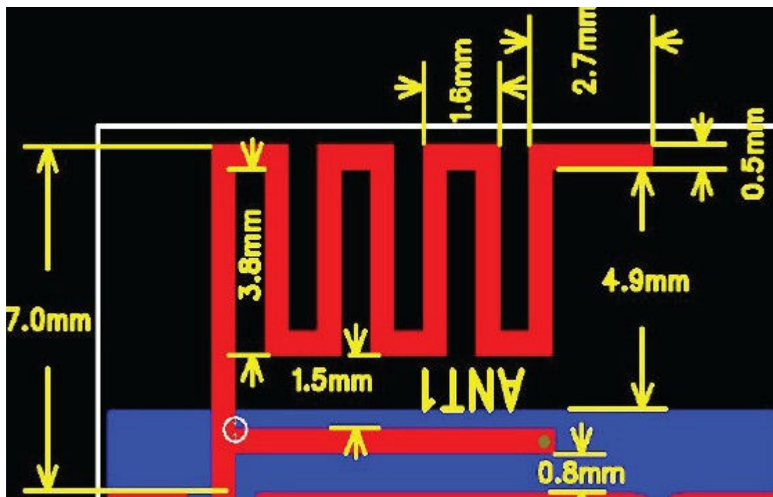
Antenna shape
