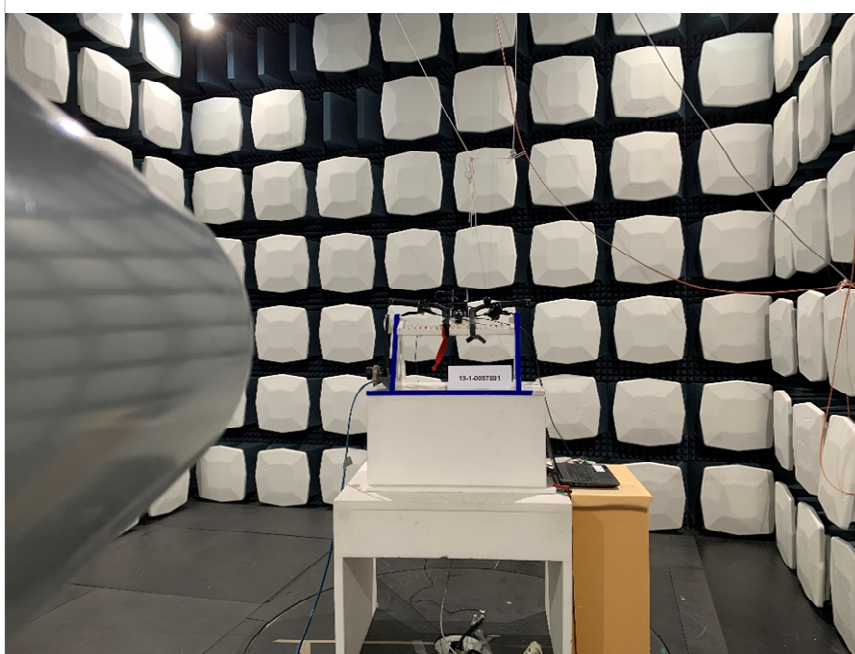
Photograph 4: EUT Setup in the fully anechoic chamber, overview
