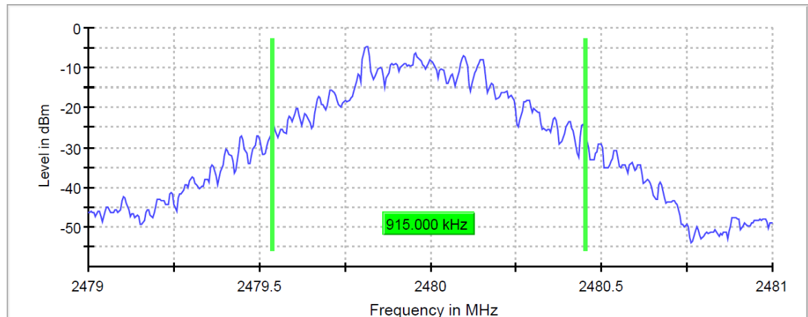
20 dB Bandwidth
