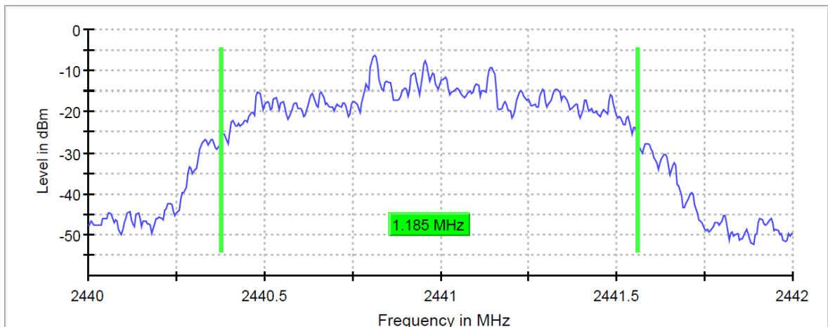
20 dB Bandwidth
