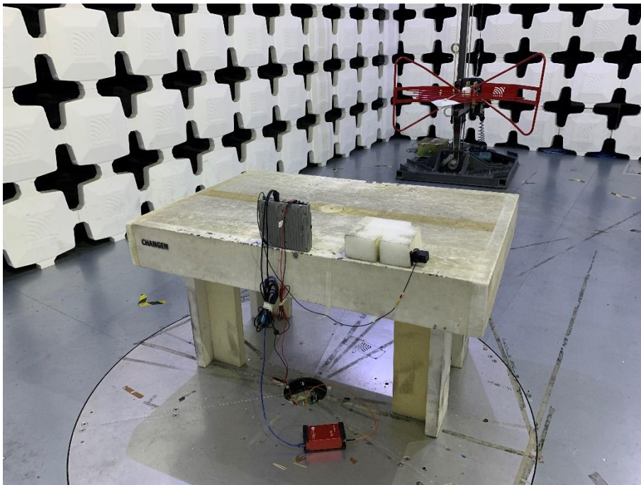
6. Radiated Emissions (Part 15C&Part 15E,30MHz-1GHz, EUT Pos 3)
