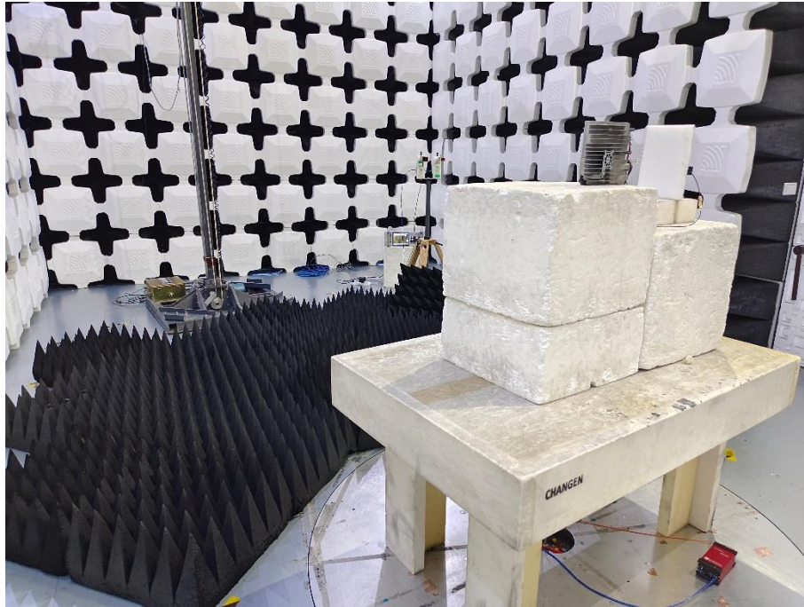
11. Radiated Emissions (Part 15C&Part 15E, 18GHz -26.5GHz, Pos 2)
