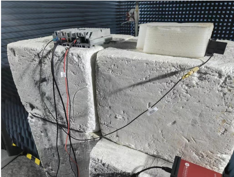
7. Radiated Emissions (Part 15C&Part 15E, 1GHz -18GHz, Pos 1)
