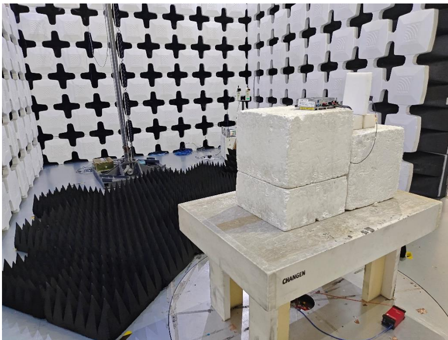
10. Radiated Emissions (Part 15C&Part 15E, 18GHz -26.5GHz, Pos 1)
