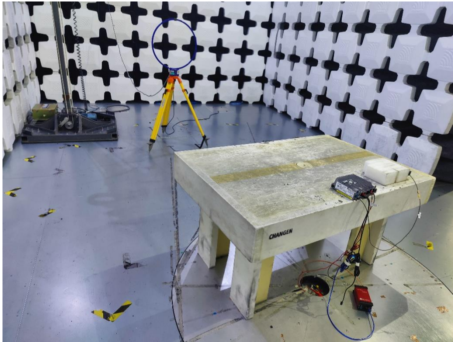
1. Radiated Emissions (Part 15C&Part 15E, 9kHz-30MHz, EUT Pos 1)
