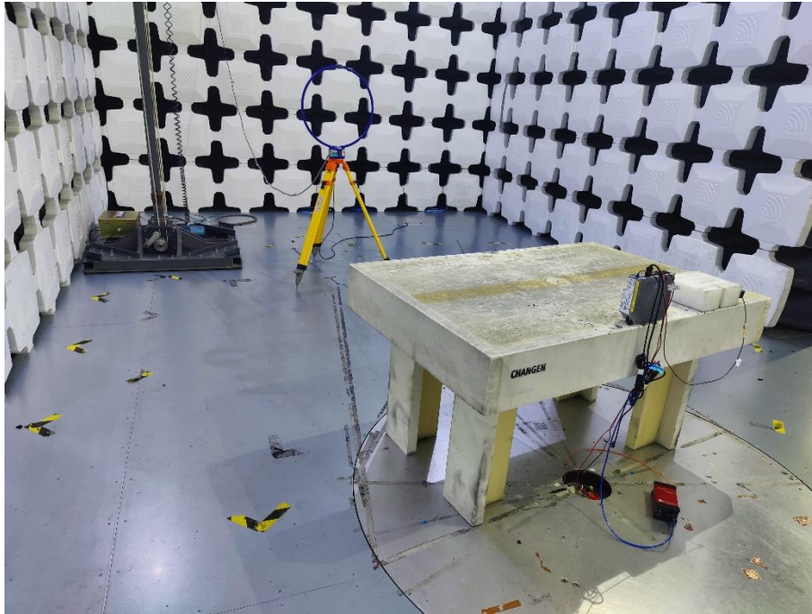
3. Radiated Emissions (Part 15C&Part 15E, 9kHz-30MHz, EUT Pos 3)
