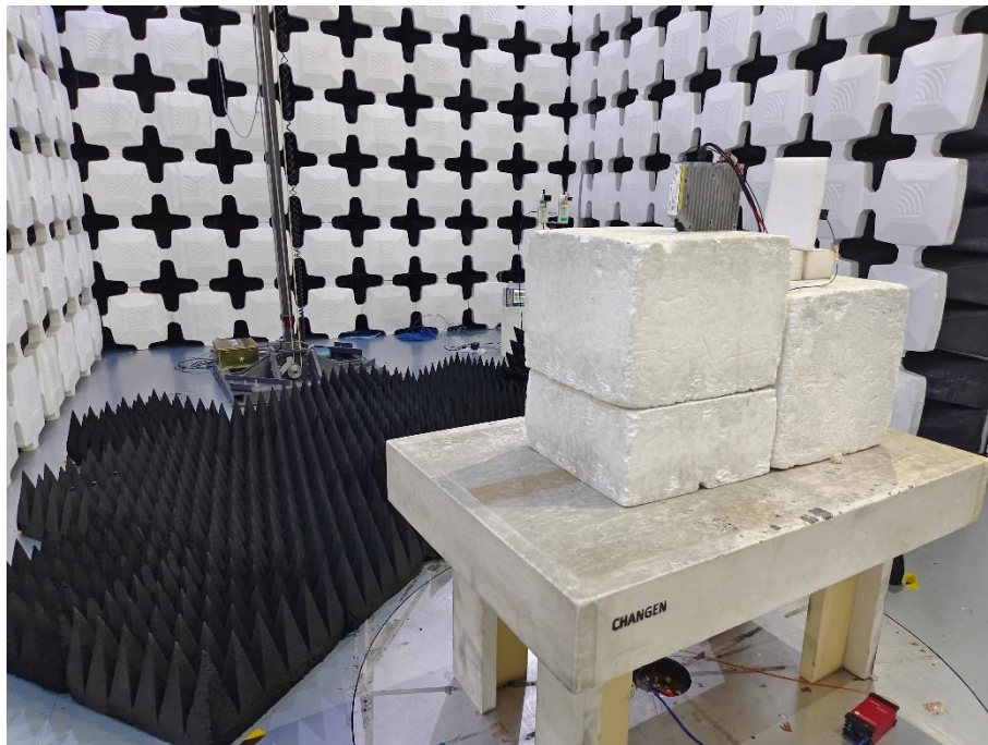
12. Radiated Emissions (Part 15C&Part 15E, 18GHz -26.5GHz, Pos 3)
