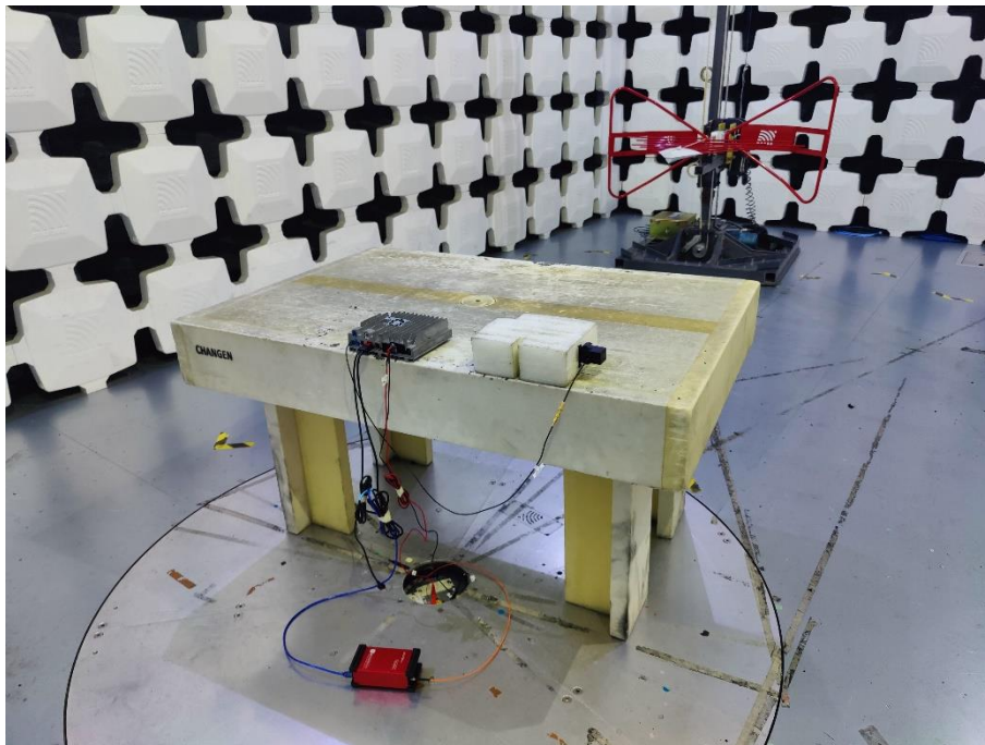
4. Radiated Emissions (Part 15C&Part 15E,30MHz-1GHz, EUT Pos 1)
