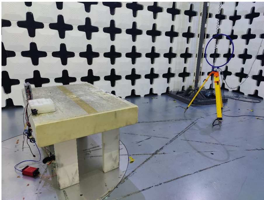
2. Radiated Emissions (Part 15C&Part 15E, 9kHz-30MHz, EUT Pos 2)
