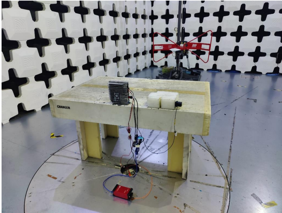
5. Radiated Emissions (Part 15C&Part 15E,30MHz-1GHz, EUT Pos 2)
