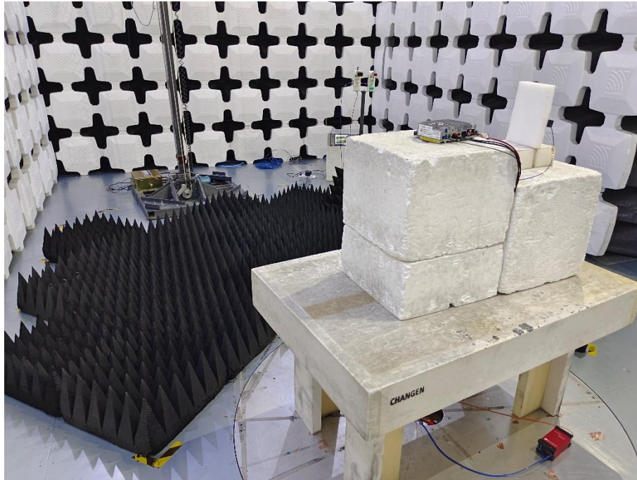
13. Radiated Emissions art 15E, 26.5GHz-40GHz, Pos 1)
