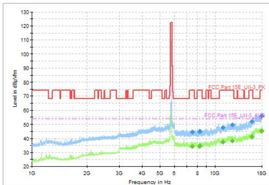
Fig. 82 Transmitter Spurious Emission (802.11n-HT40, CH151 5755MHz, 1GHz-18GHz), MIMO
