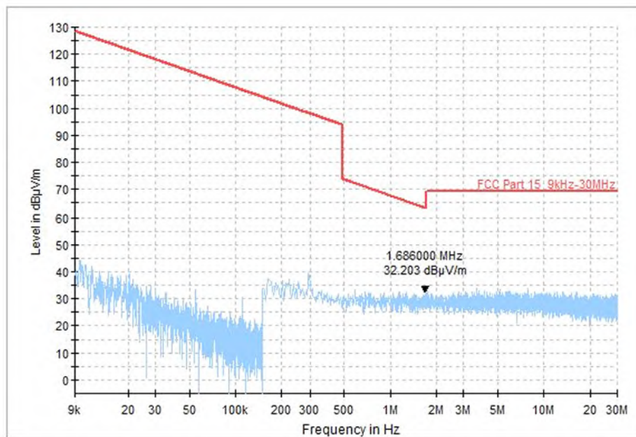
Fig. 94 Radiated Spurious Emission (All Channel, 9 kHz ~30 MHz), MIMO
