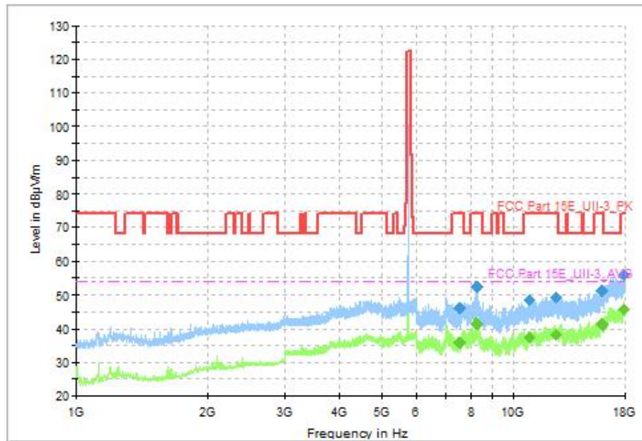
Fig. 77 Transmitter Spurious Emission (802.11ax-HE20, CH149 5745MHz, 1GHz-18GHz), MIMO
