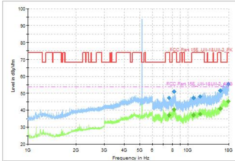
Fig. 49 Transmitter Spurious Emission (802.11ax-HE20, CH36 5180MHz, 1GHz-18GHz)
