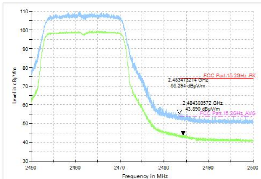
Fig.88 Radiated Restricted Band (802.11n-HT20, CH11, 2.45GHz~2.50GHz),MIMO
