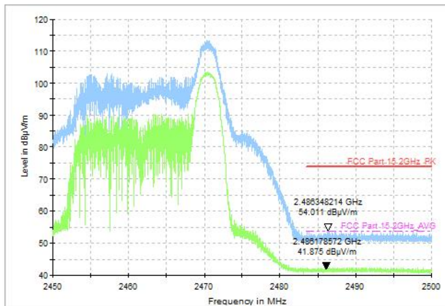
Fig.80 Radiated Restricted Band (802.11ax-HE20, CH11(RU26), 2.45GHz~2.50GHz)
