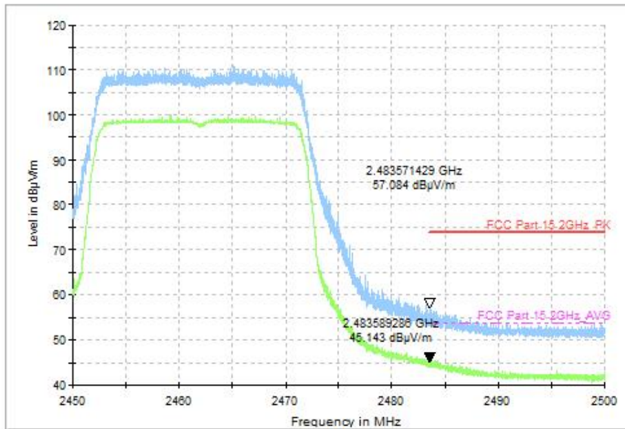
Fig.93 Radiated Restricted Band (802.11ax-HE20, CH11, 2.45GHz~2.50GHz),MIMO
