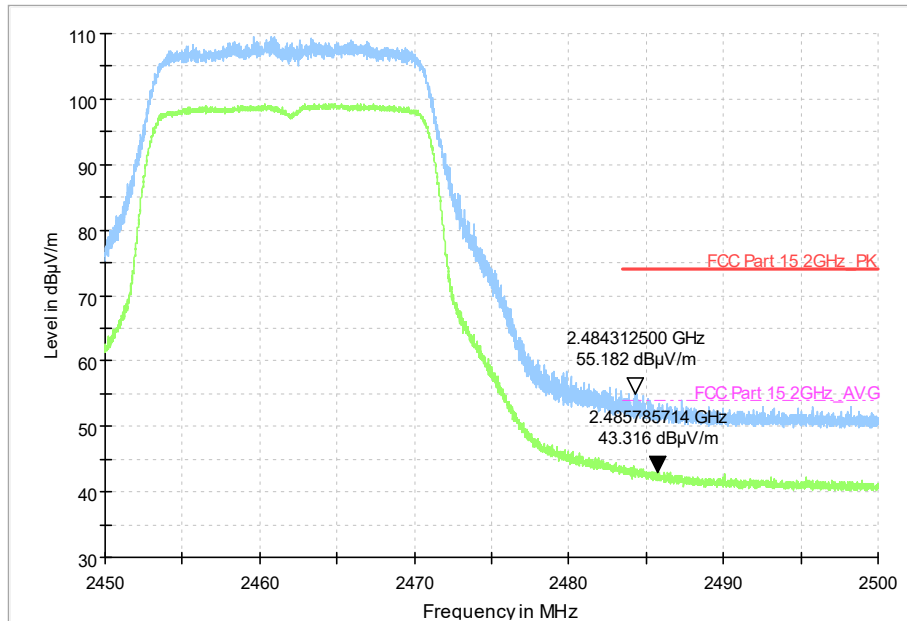
Fig.71 Radiated Restricted Band (802.11n-HT20, CH11, 2.45GHz~2.50GHz)
