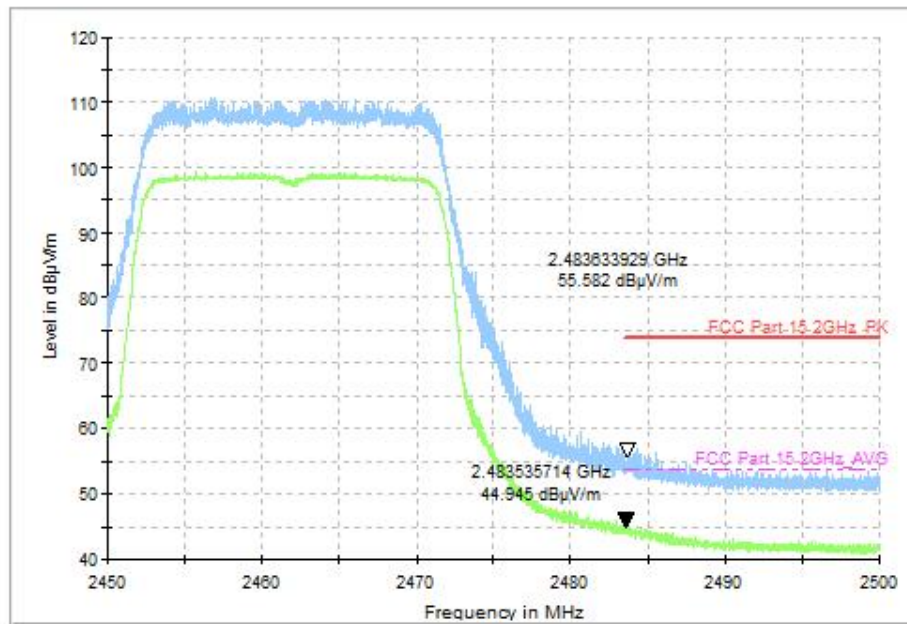
Fig.76 Radiated Restricted Band (802.11ax-HE20, CH11, 2.45GHz~2.50GHz)
