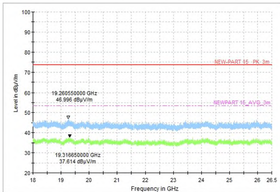
Fig.96 Radiated Spurious Emission (All channel, 18GHz~26.5GHz),MIMO
