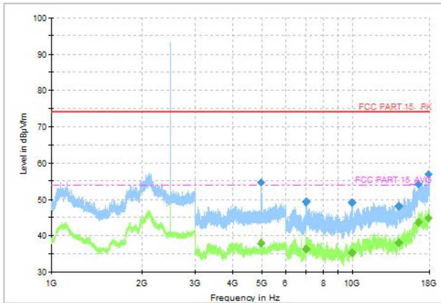
Fig.32 Radiated Spurious Emission (CH39, 1GHz ~18GHz), LE 1M
