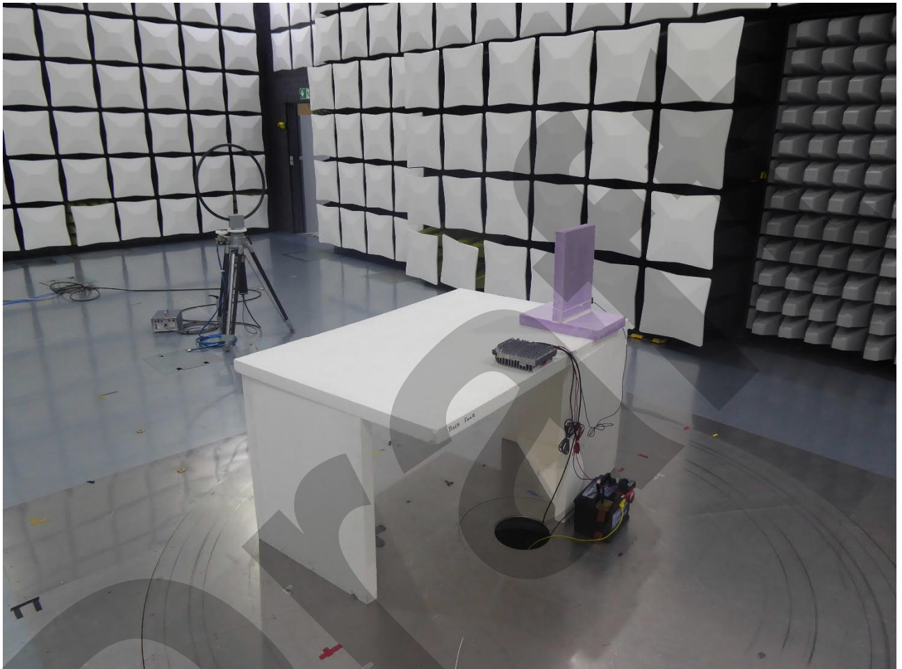
Test setup semi anechoic chamber (9 kHz – 30 MHz) – EUT Pos 1
