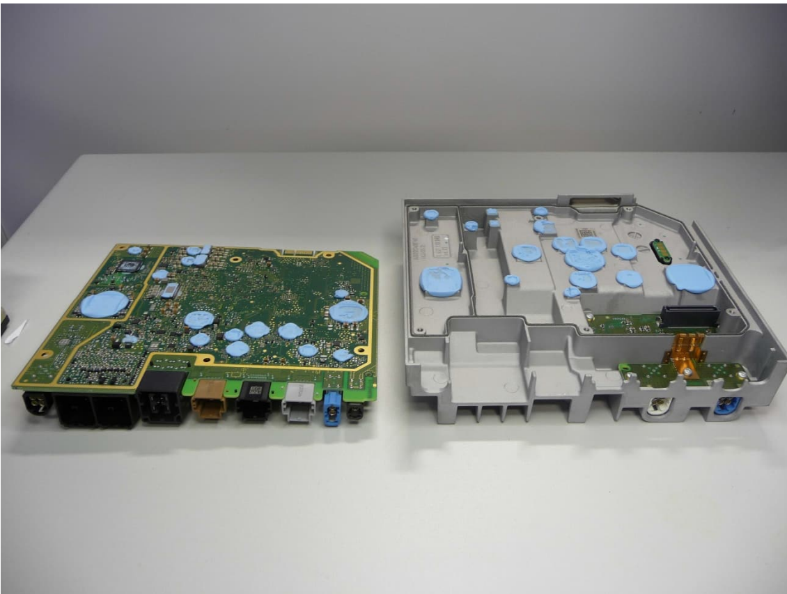
PCB removed
