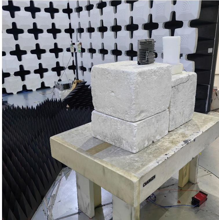
11. Radiated Emissions (Part 15C&Part 15E, 18GHz -26.5GHz, Pos 2)
