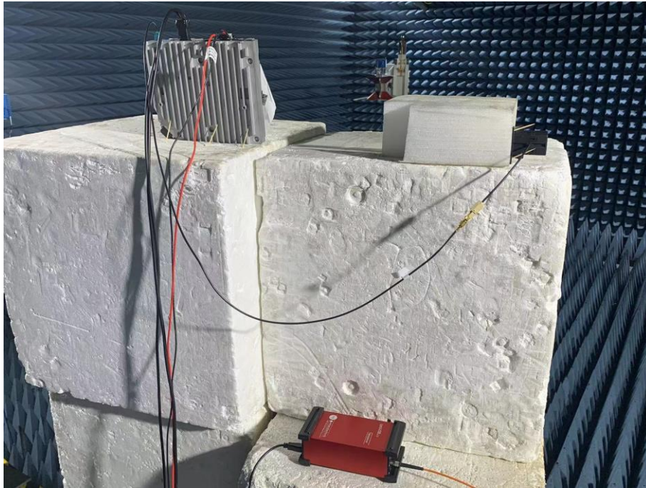
9. Radiated Emissions (Part 15C&Part 15E, 1GHz -18GHz, Pos 3)
