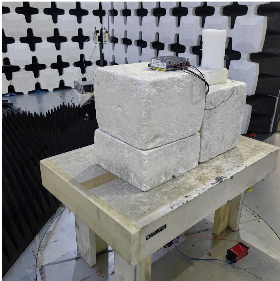
10. Radiated Emissions (Part 15C&Part 15E, 18GHz -26.5GHz, Pos 1)
