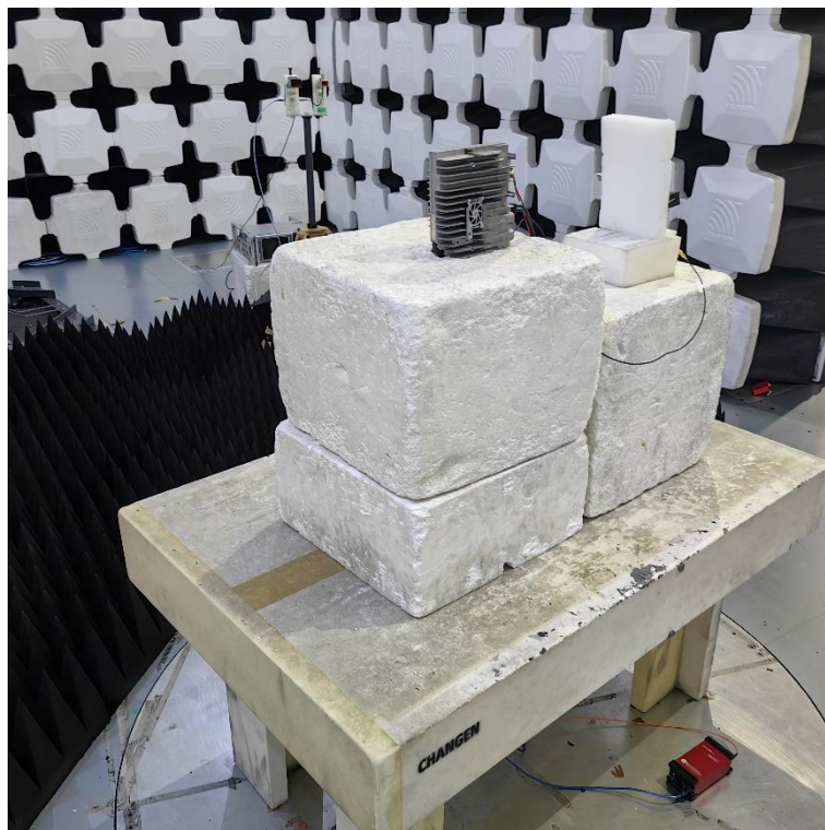
14. Radiated Emissions art 15E, 26.5GHz-40GHz, Pos 2)
