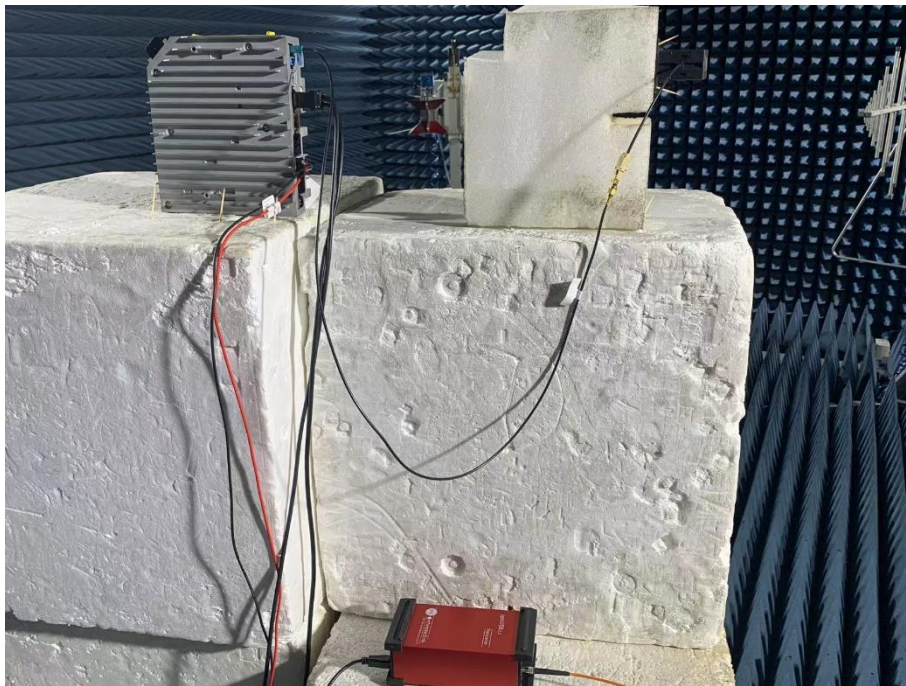
8. Radiated Emissions (Part 15C&Part 15E, 1GHz -18GHz, Pos 2)
