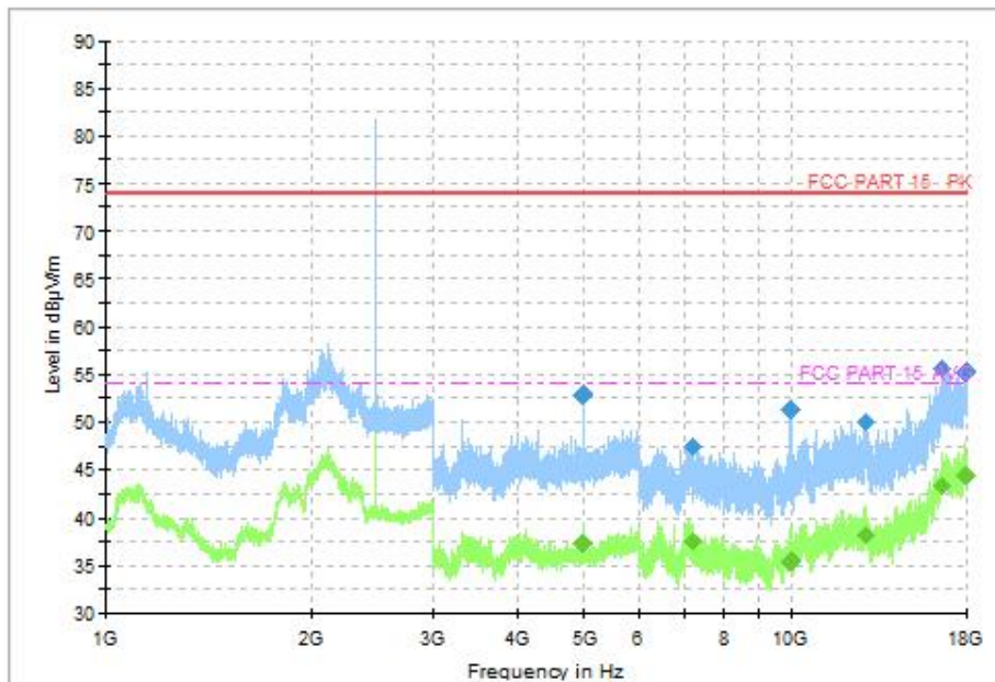
Fig.37 Radiated Spurious Emission (CH39, 1GHz ~18GHz), LE 2M
