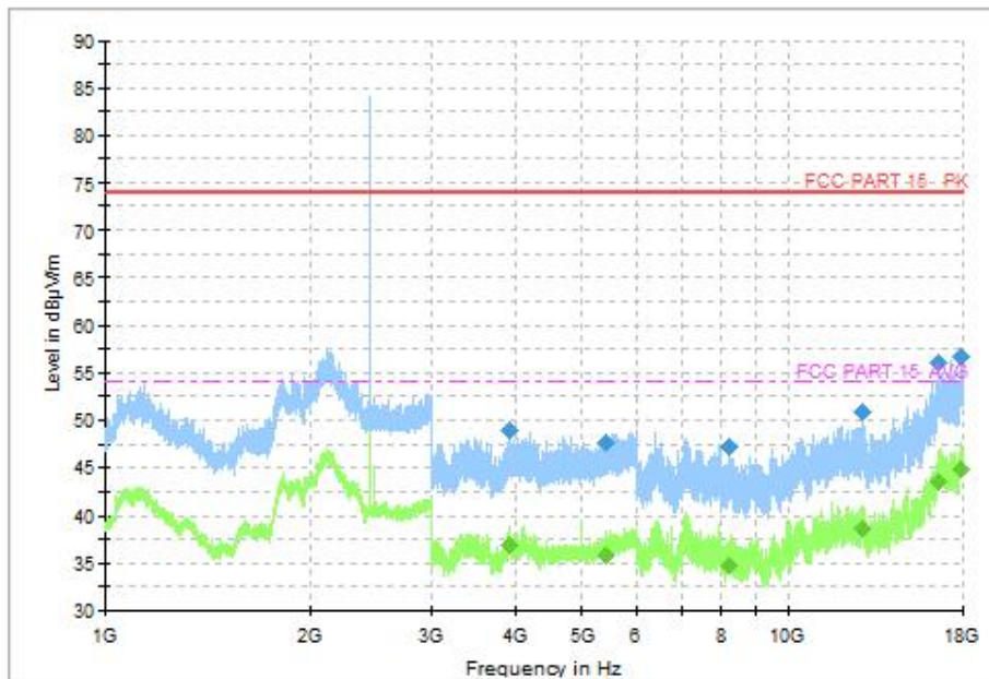
Fig.31 Radiated Spurious Emission (CH19, 1GHz ~18GHz), LE 1M
