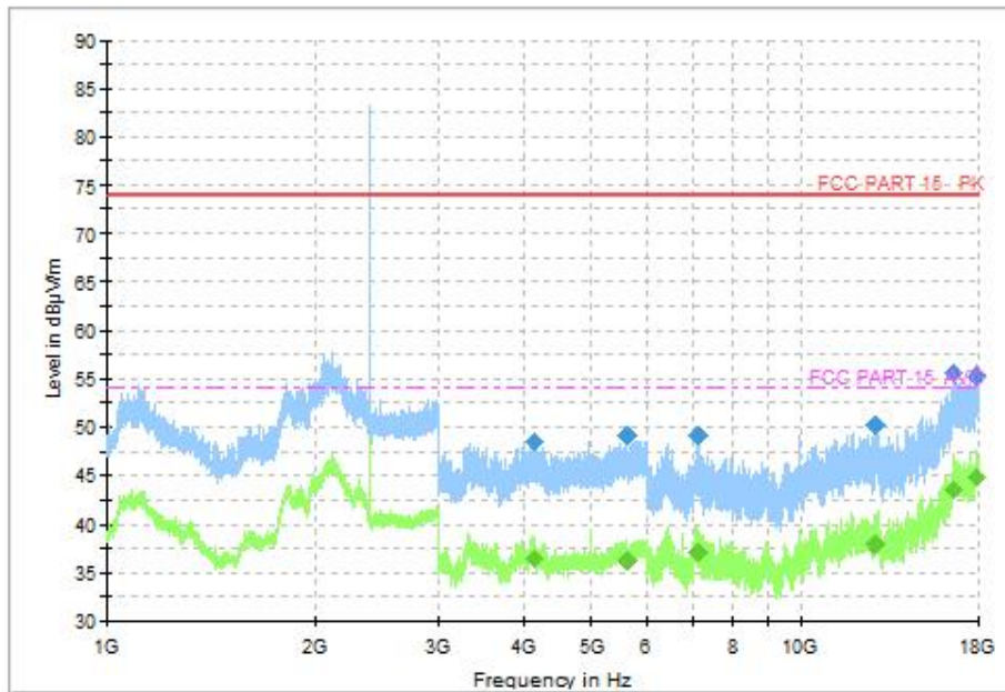
Fig.30 Radiated Spurious Emission (CH0, 1GHz ~18GHz), LE 1M
