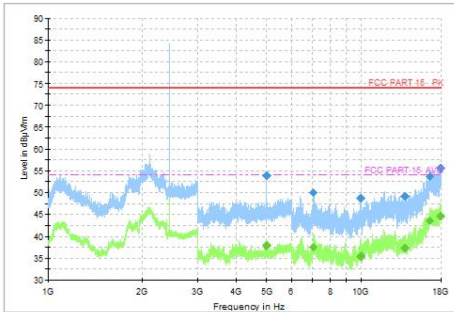
Fig.36 Radiated Spurious Emission (CH19, 1GHz ~18GHz), LE 2M
