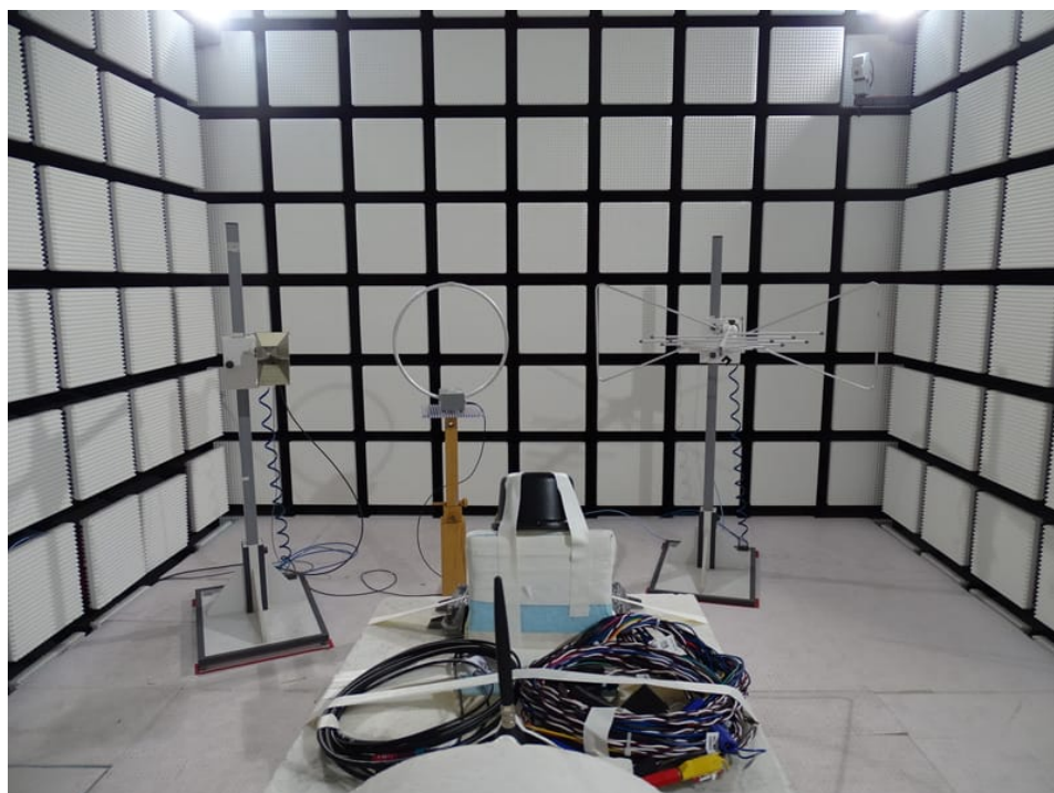
Photo 13: RSE tests with Puck antenna
