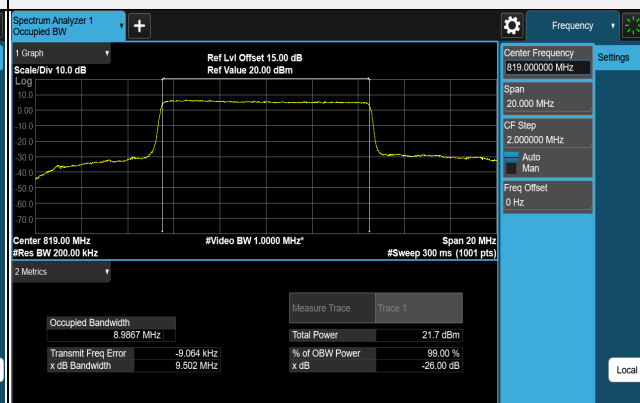
64QAM CH 26740 (819MHz)
