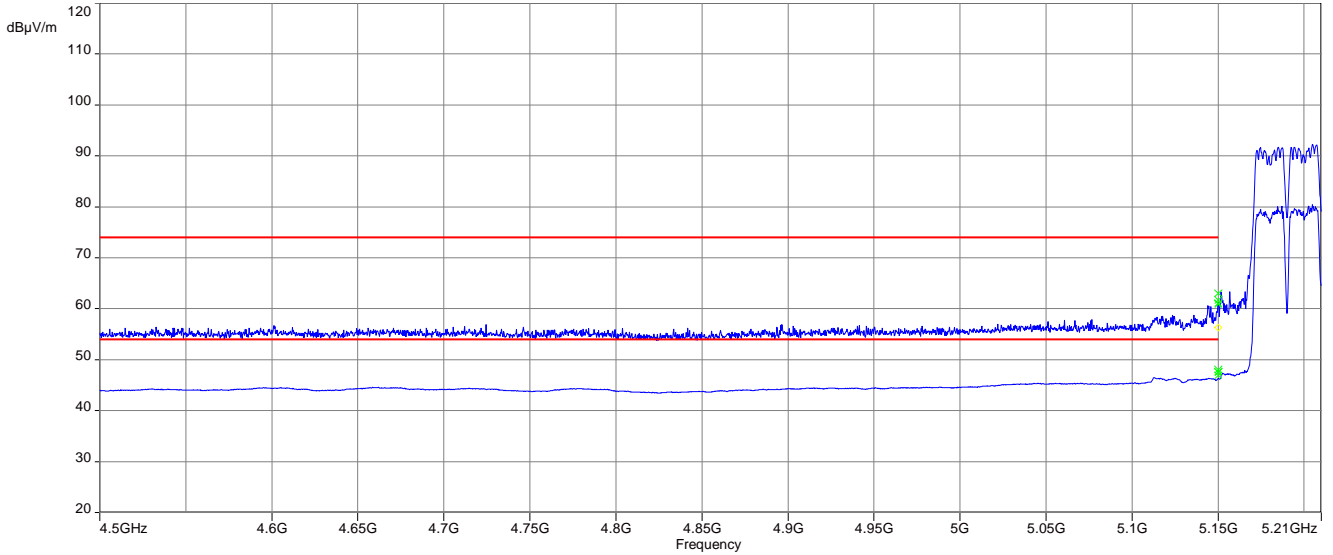
Plot 7: lower band edge; U-NII-1; middle channel; 80 MHz channel bandwidth
