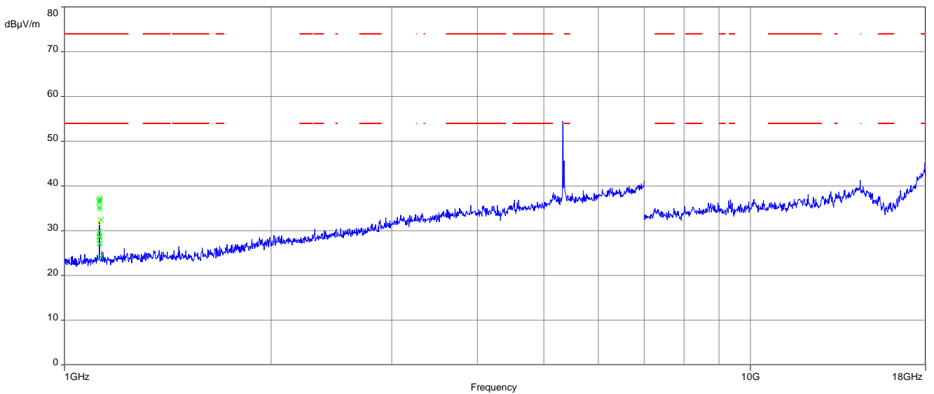
Plot 2: 1 GHz to 18 GHz; vertical & horizontal polarization; U-NII-2A; highest channel
