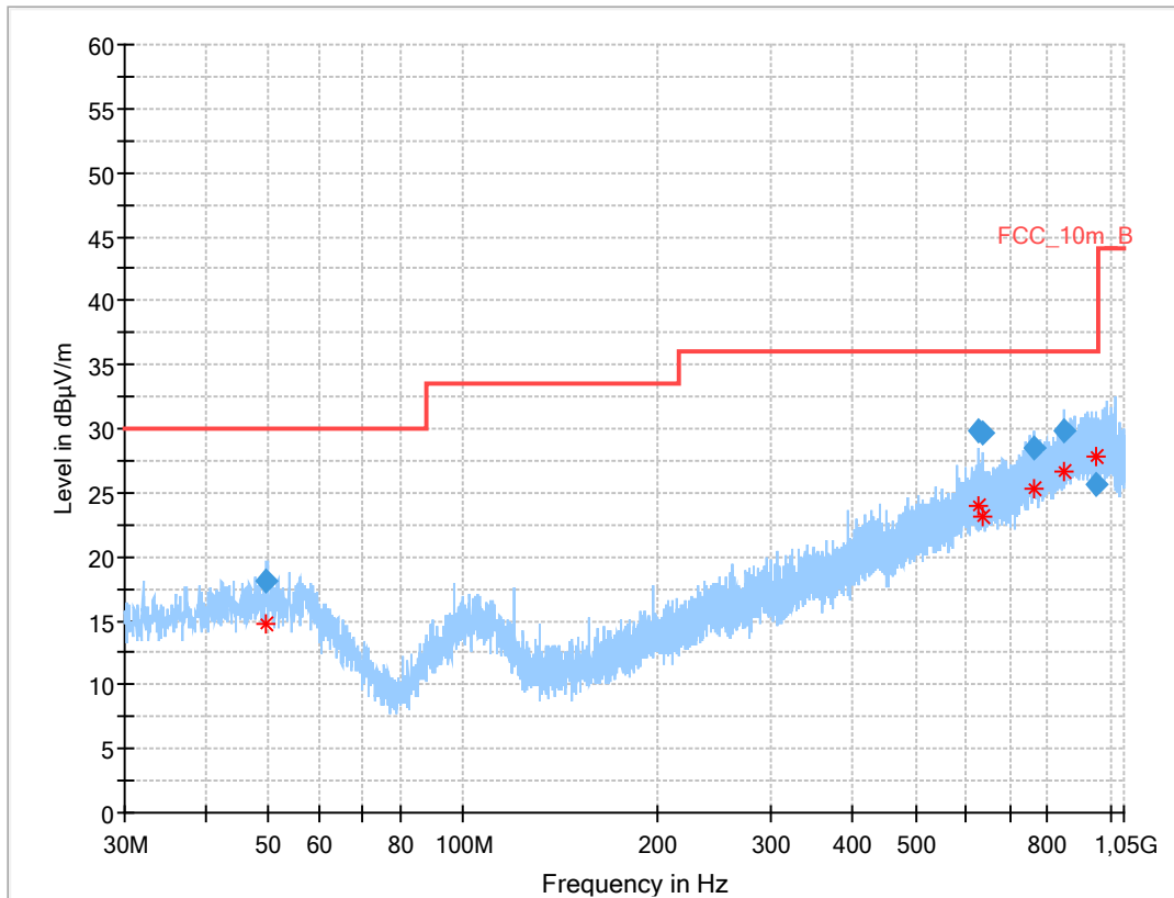
Plot 1: 30 MHz to 1 GHz; vertical & horizontal polarization; U-NII-2A; valid for all channels and modes
