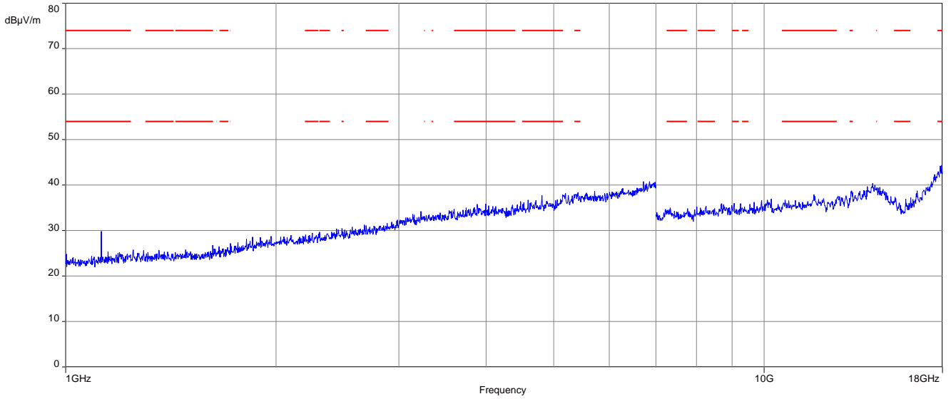
Plot 1: 1 GHz to 18 GHz; vertical & horizontal polarization; U-NII-2A; lowest channel
