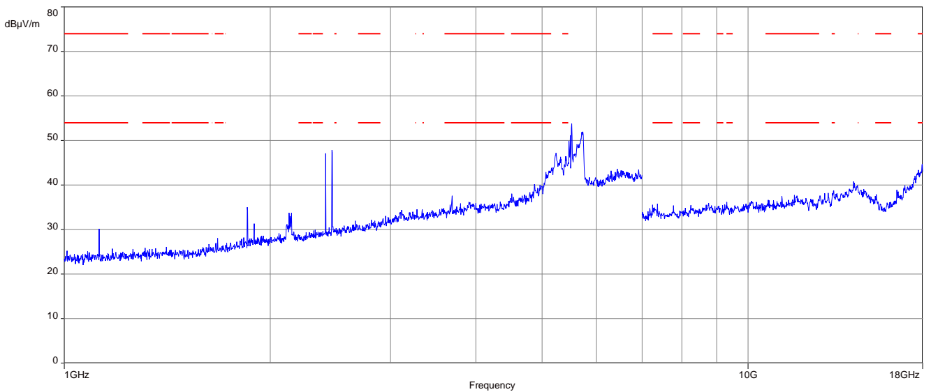
Plot 2: 1 GHz to 18 GHz; vertical & horizontal polarization; U-NII-2C; lowest channel
