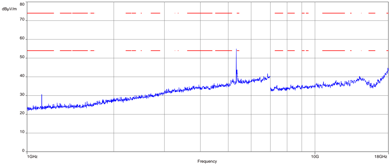
Plot 1: 1 GHz to 18 GHz; vertical & horizontal polarization; U-NII-2A; middle channel
