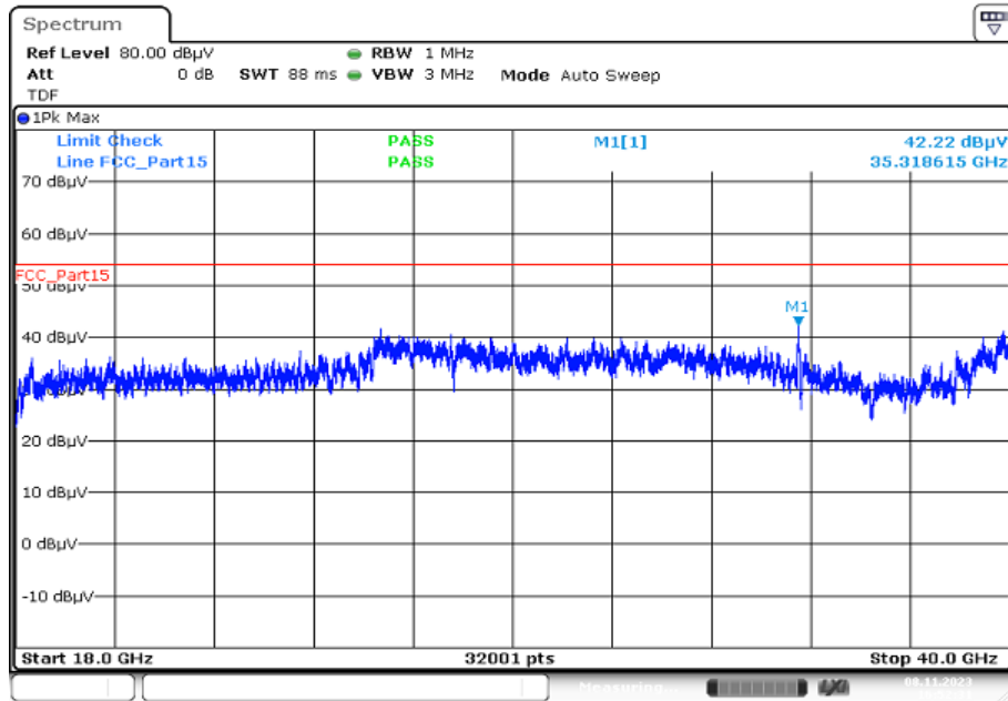
Plot 3: 18 GHz to 40 GHz; vertical & horizontal polarization; valid for all bands, modes and channels
