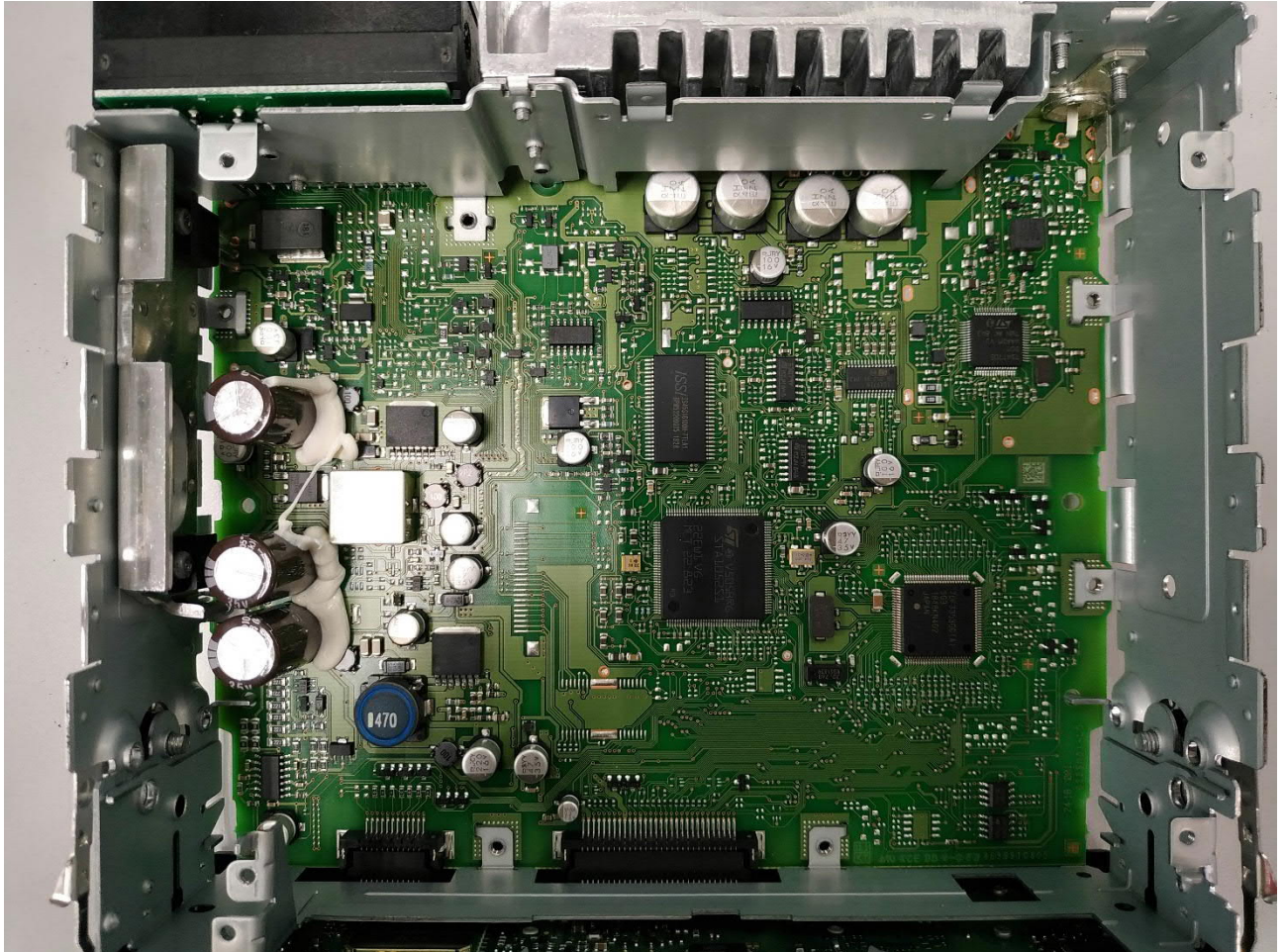
Main PCB – top view / Internal view*
