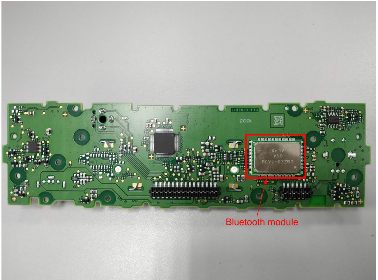
Display PCB – bottom view*
