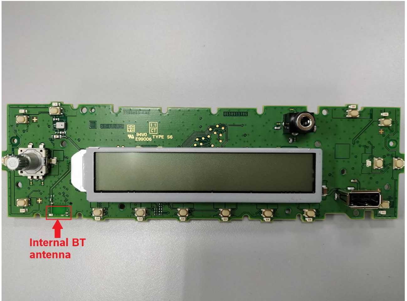
Display PCB – top view*
