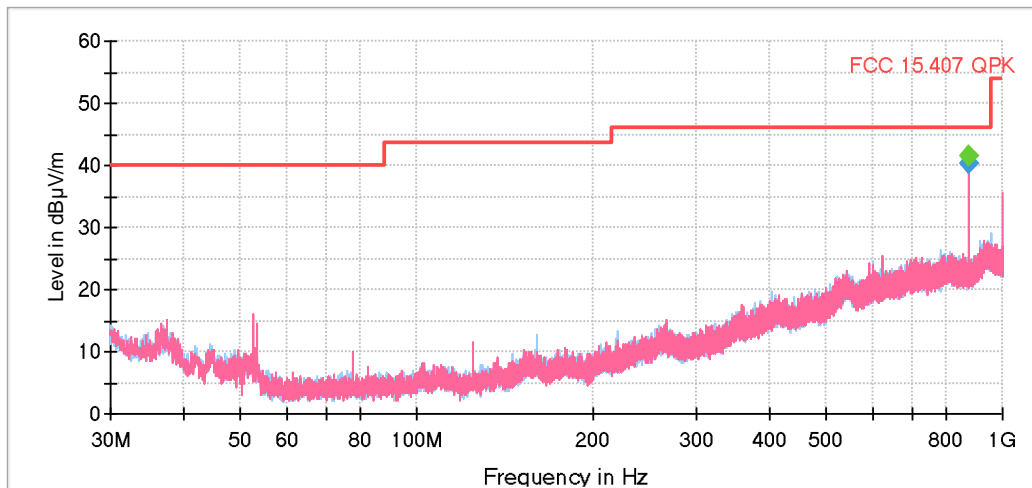
◆ Preview Result 1H-PK+ Final_Result QPK ◆ Preview Result 1V-PK+ Final_Result PK+ — FCC 15.407 QPK
