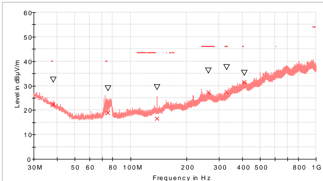
RF_FCC_15.407_E Field_30MHz_1GHz
