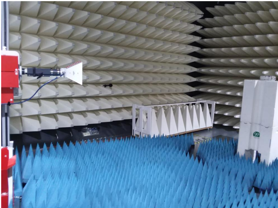
Figure C2. High Range Radiated Emission test setup 1-18GHz
