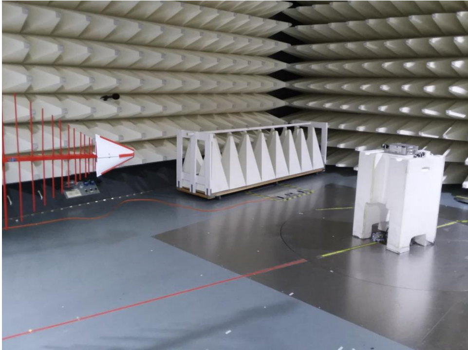
Figure C1. Low Range Radiated Emission test setup
