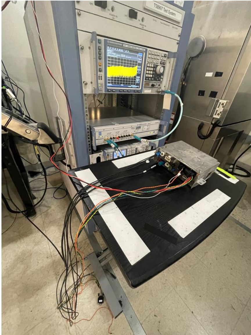
Figure C4. Conducted setup
