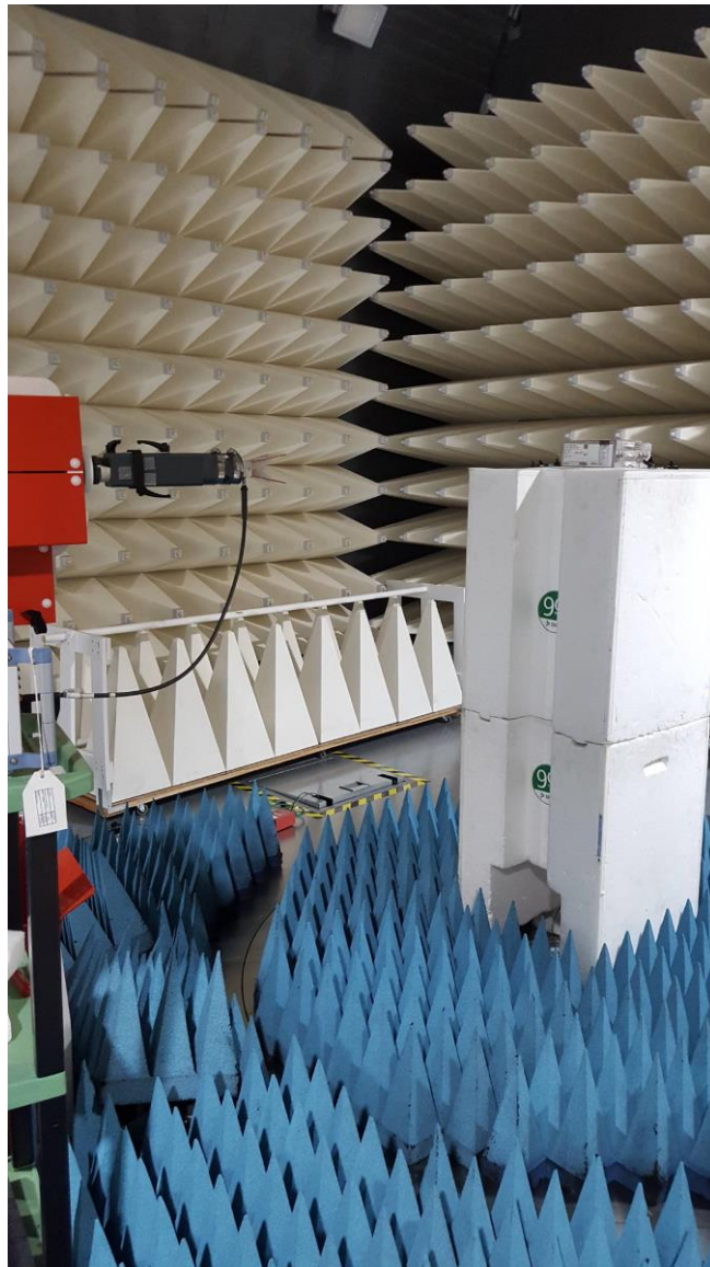
Figure C3. High Range Radiated Emission test setup 18-40GHz
