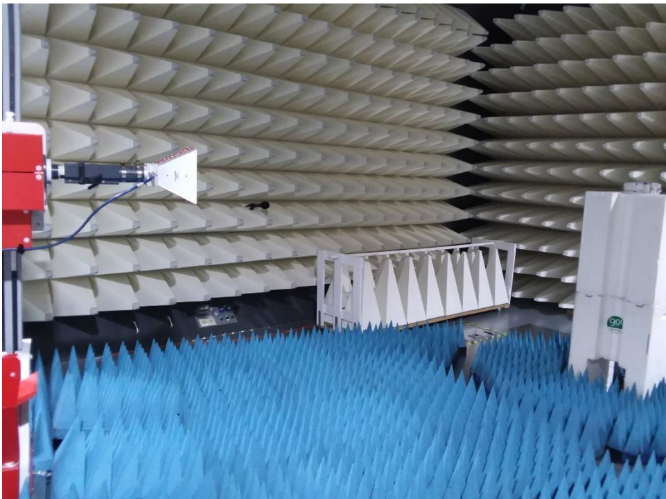
Figure B2. High Range Radiated Emission test setup 1-18GHz
