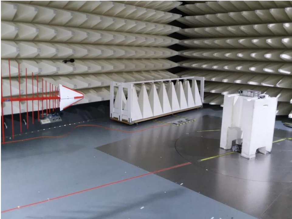
Figure B1. Low Range Radiated Emission test setup
