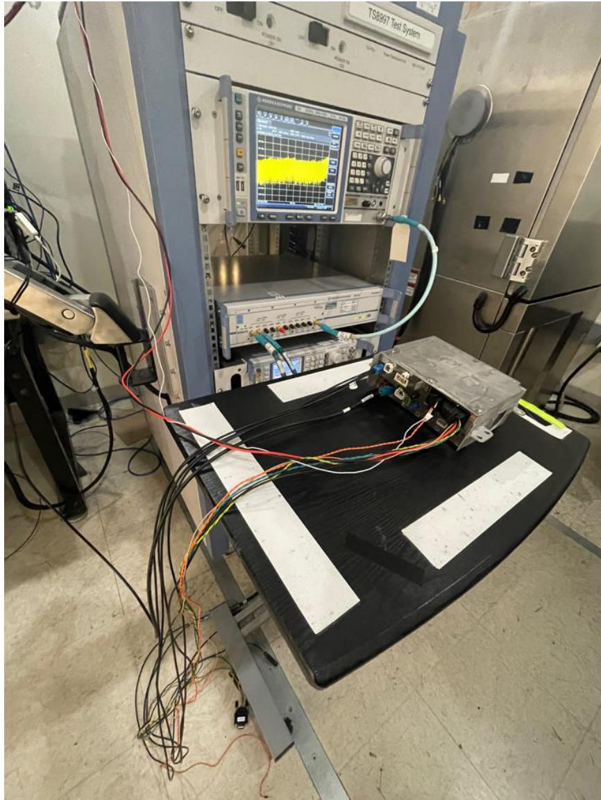
Figure B4. Conducted setup
