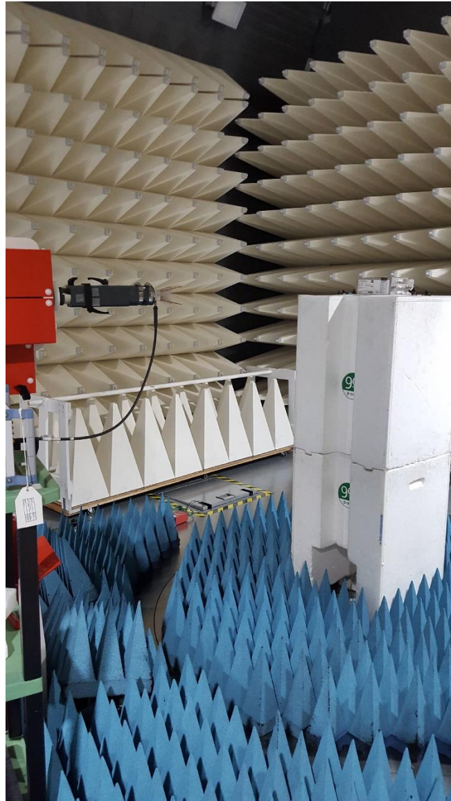
Figure B3. High Range Radiated Emission test setup 18-40GHz
