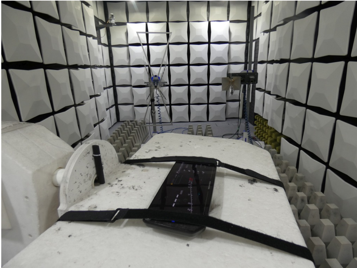
Photo 7: Setup for radiated emissions > 1 GHz, detailed view
