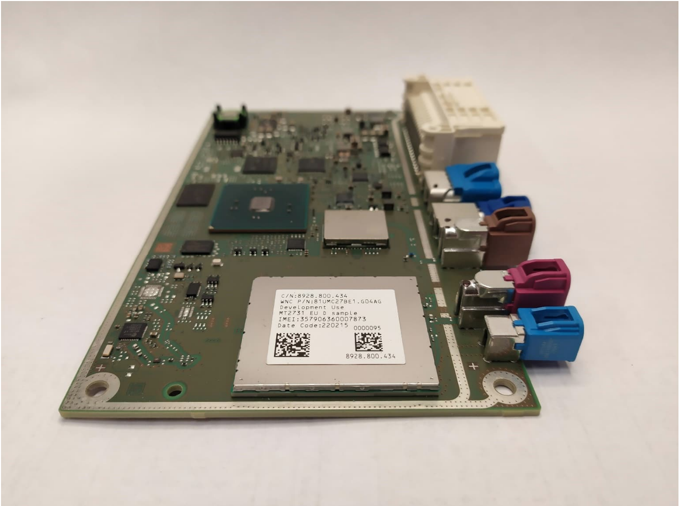
EUT internal – top view left*
