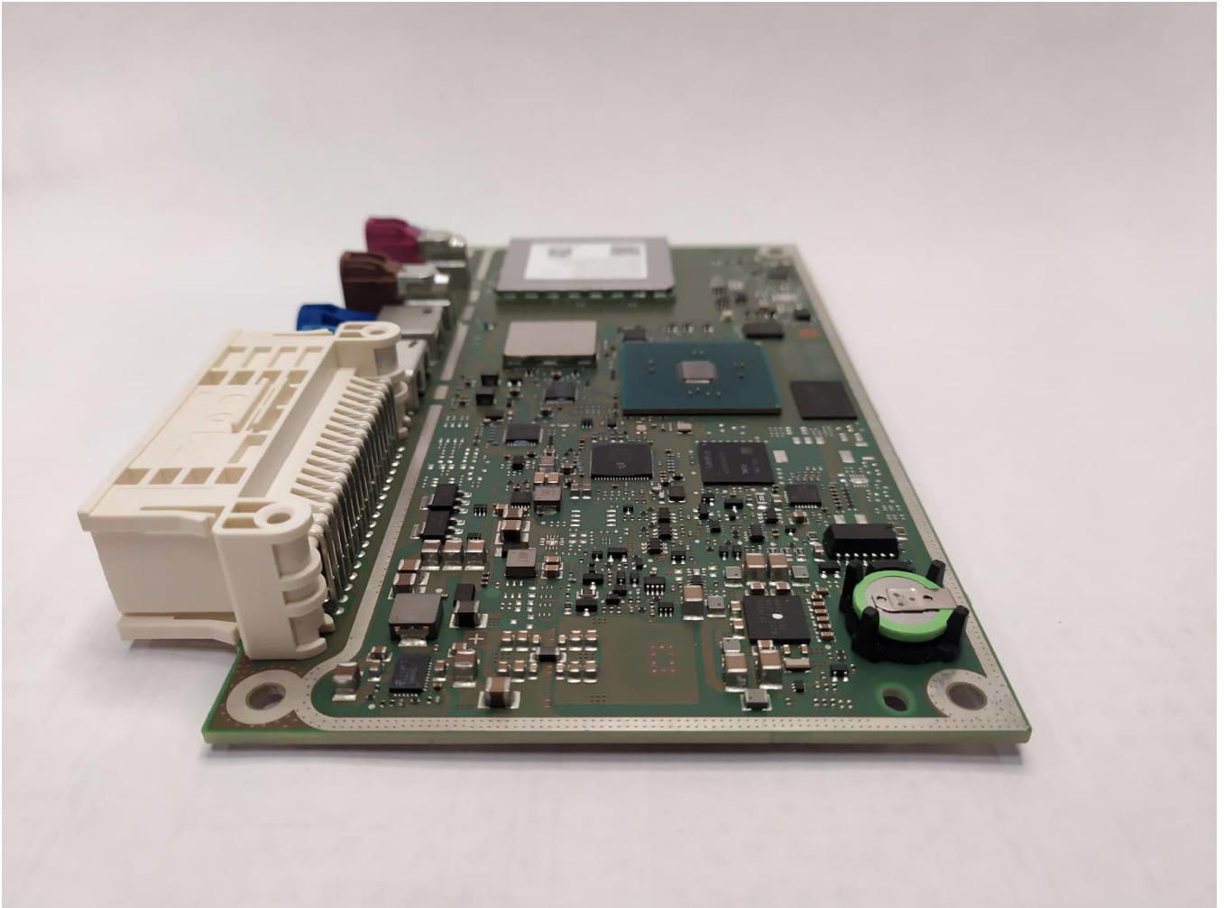
EUT internal – top view right*
