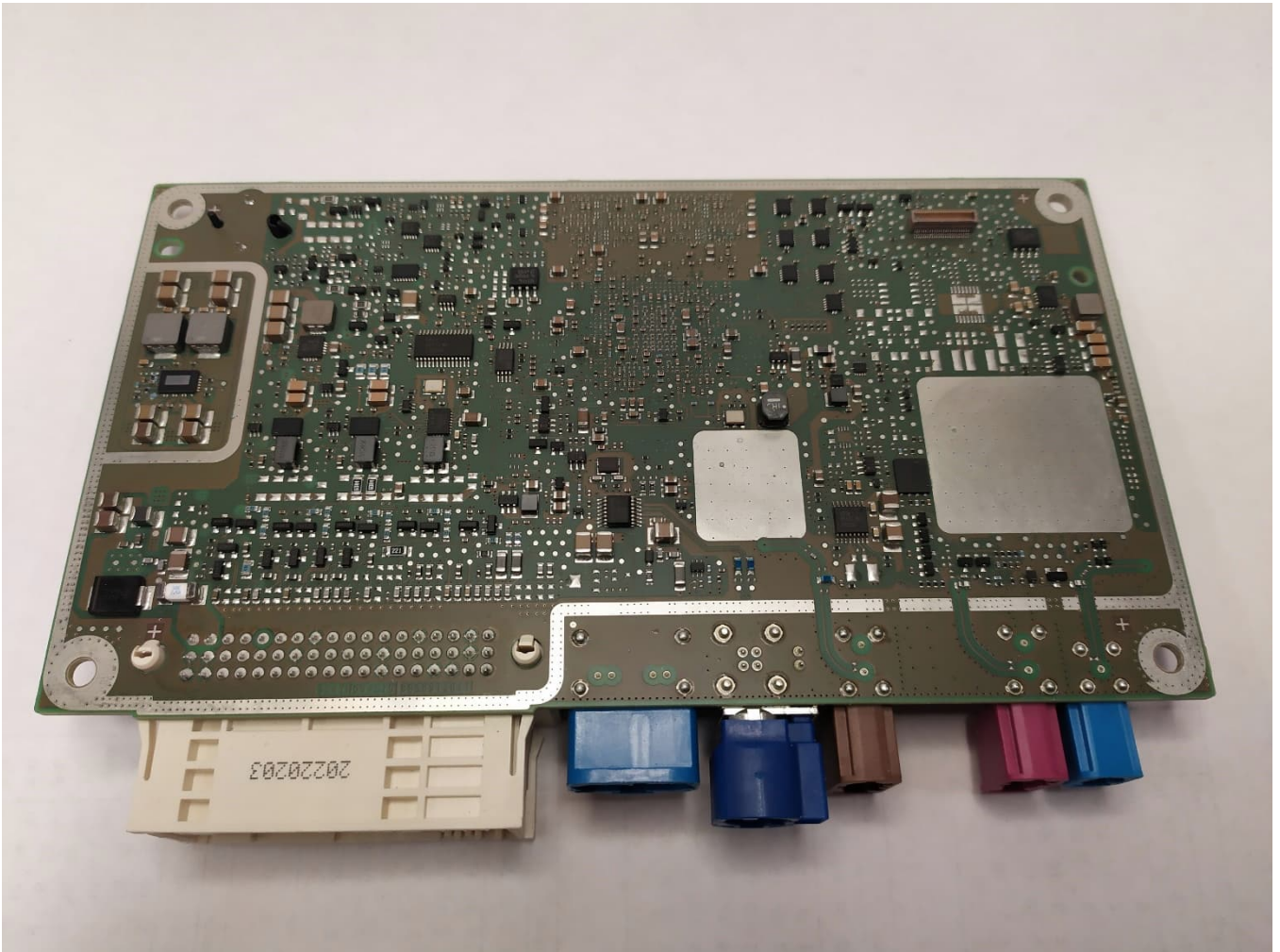
EUT internal – bottom view*
