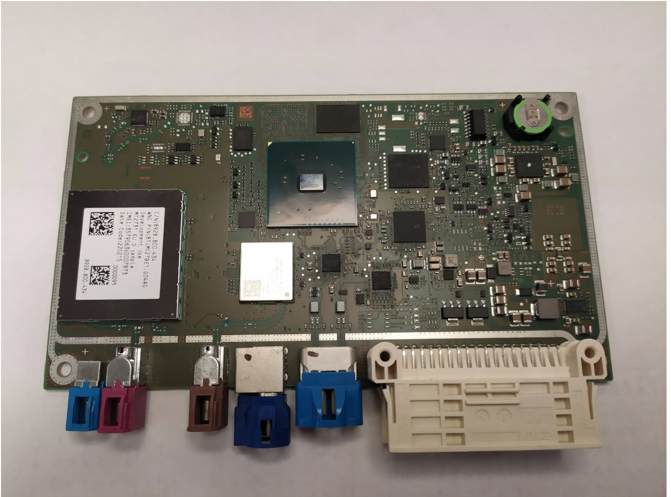
EUT internal – top view 3*
