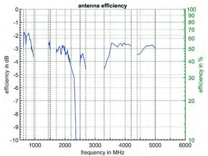
Efficiency (incl. Filtering)
