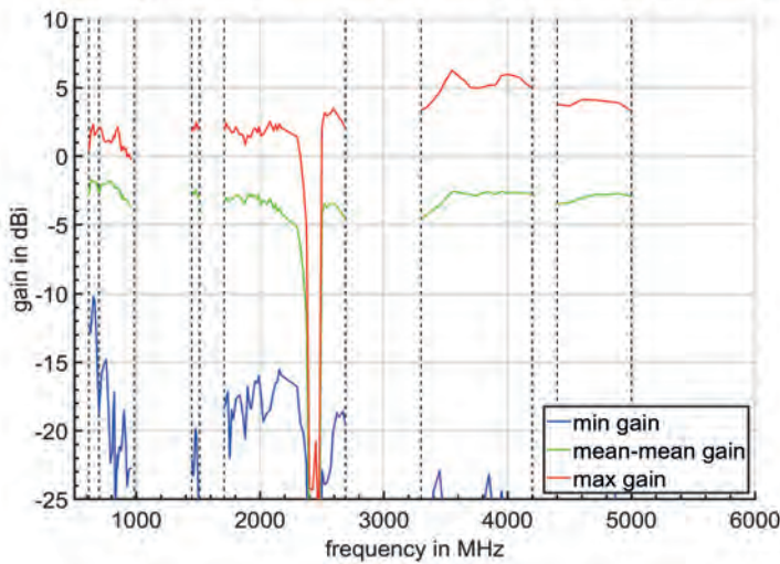
Average Gain
