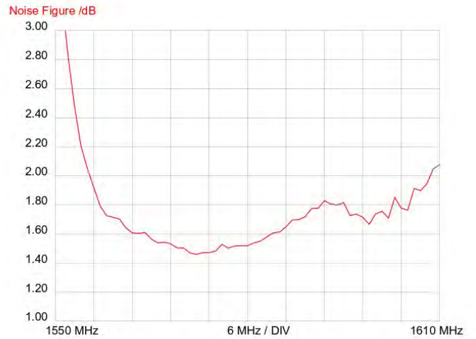
LNA Noise Figure
