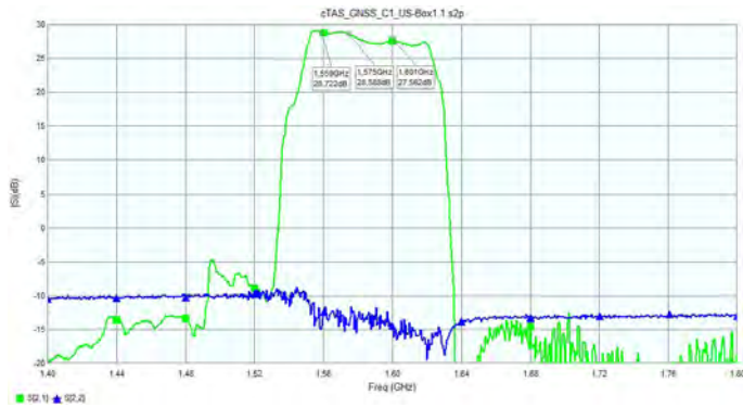
LNA Gain
