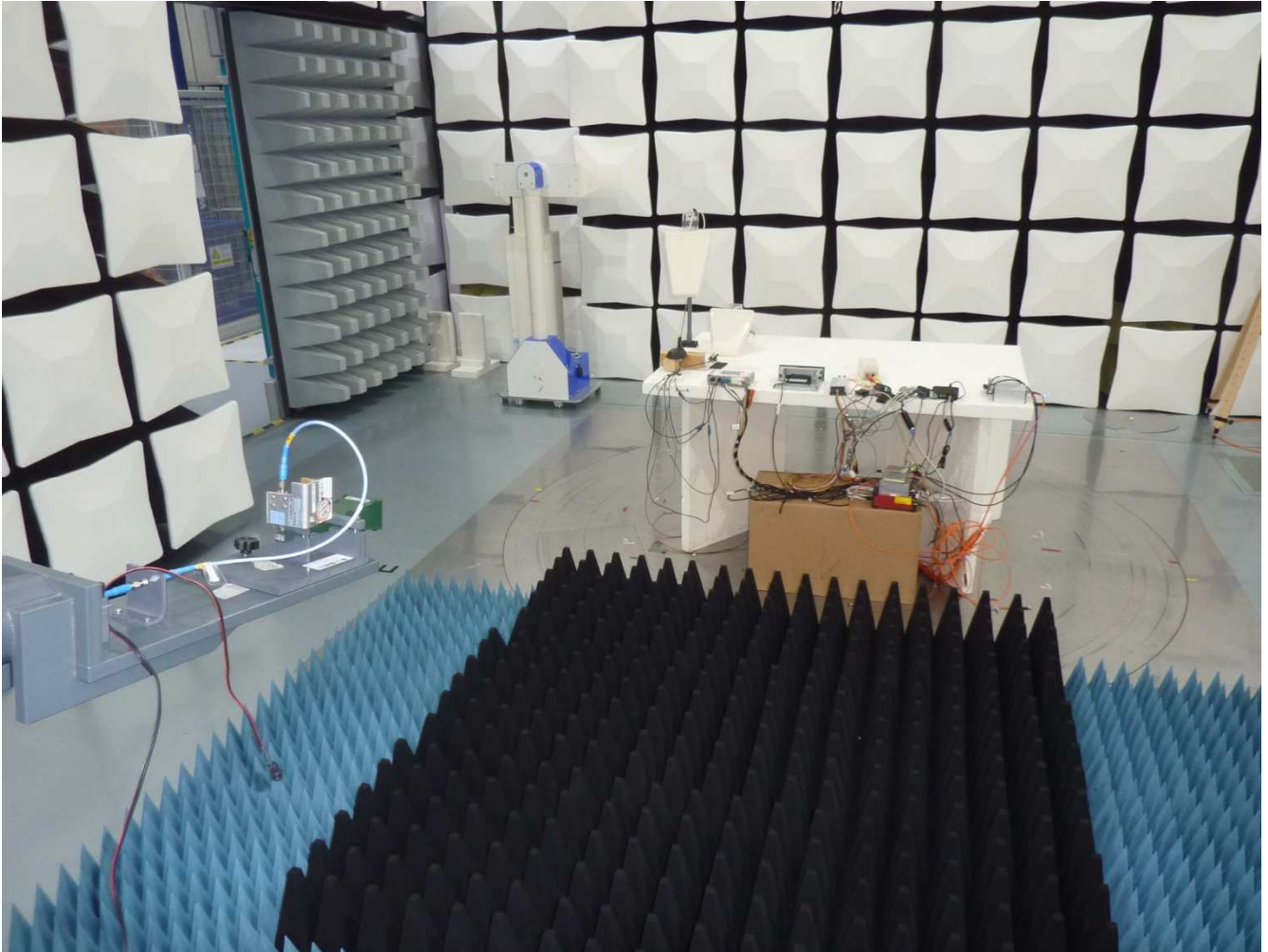
Setup 18 GHz – 26.5 GHz
