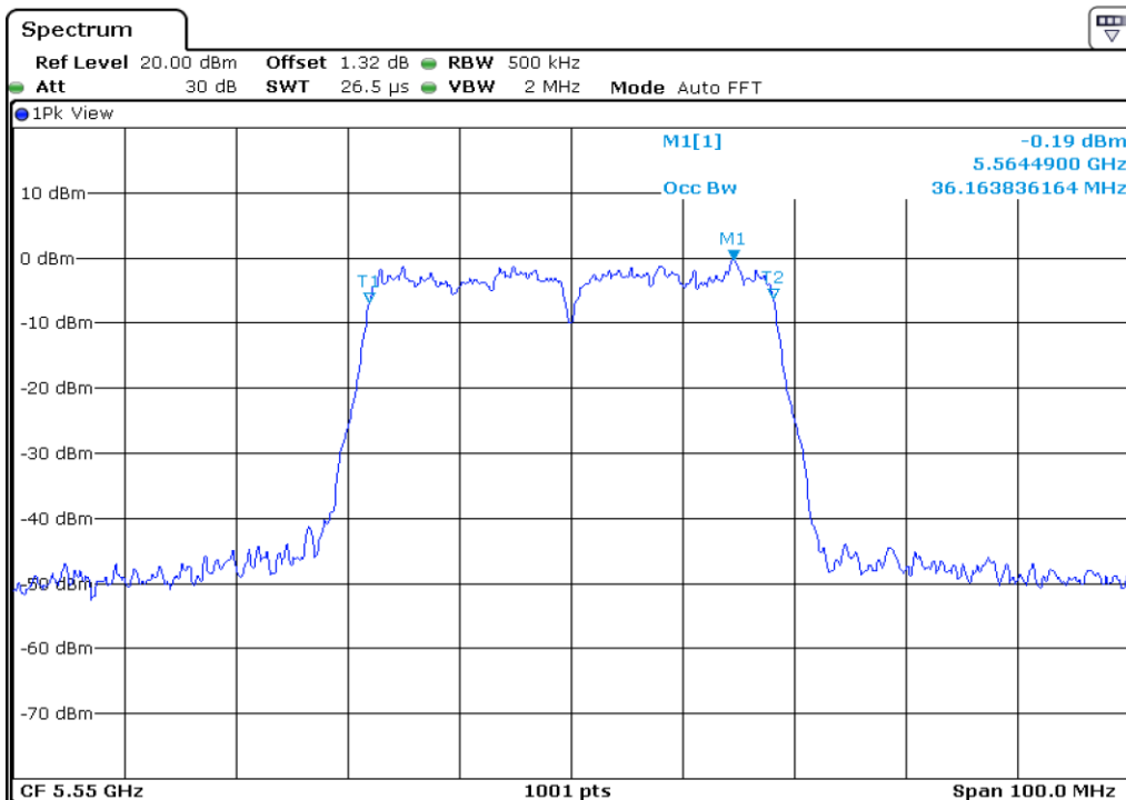
8 99% Occupied Bandwidth
