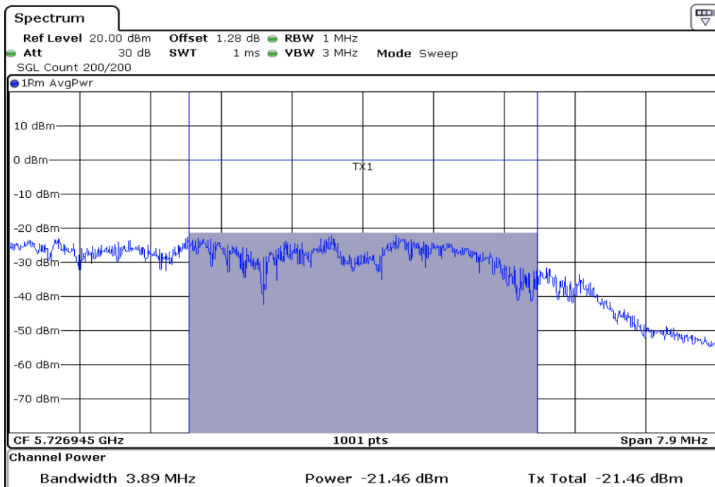
4 Starddle Maximum Conducted Output Power_UNII3
