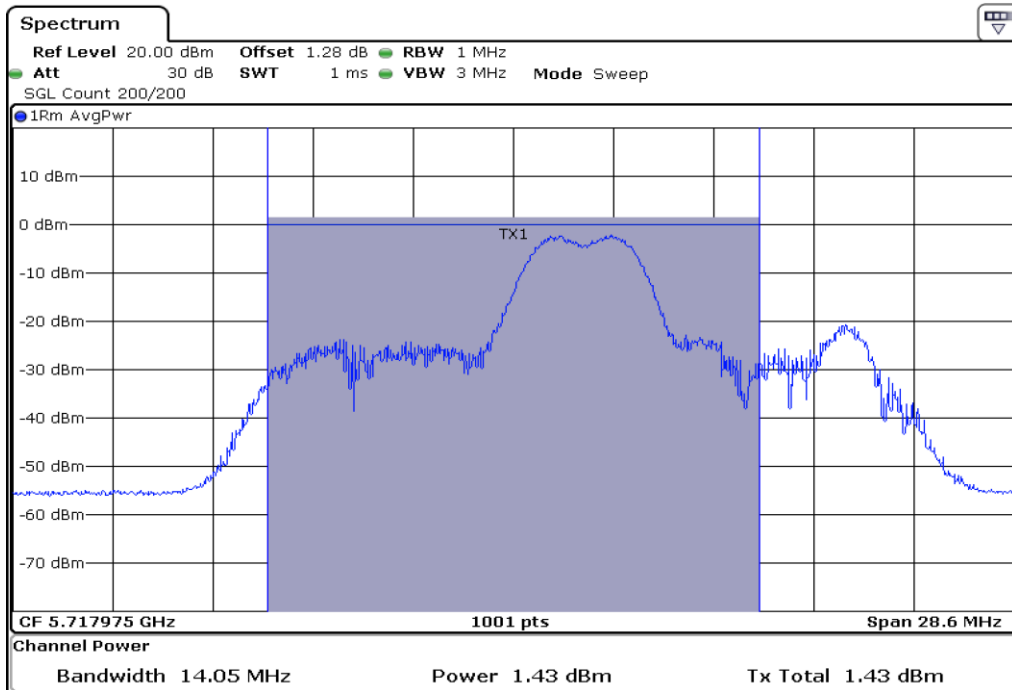
3 Starddle Maximum Conducted Output Power_UNII2C
