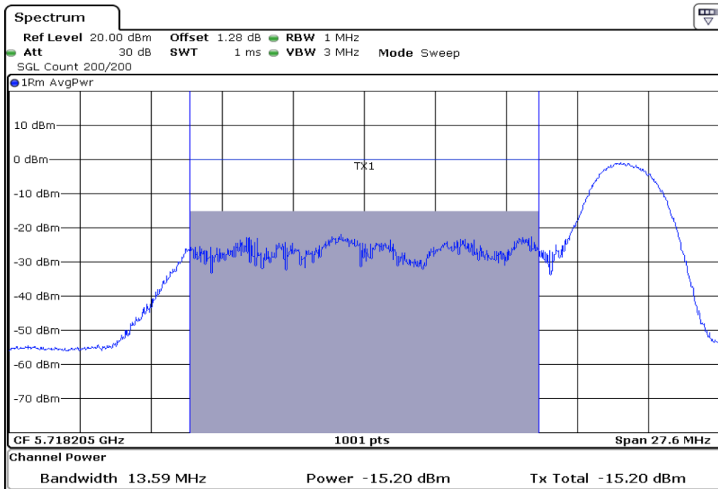
5 Starddle Maximum Conducted Output Power_UNII2C
