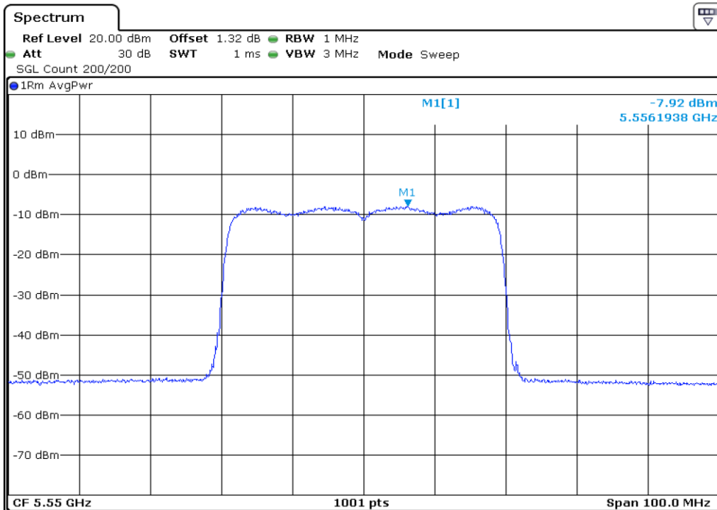
35 Peak Power Spectrul Density
