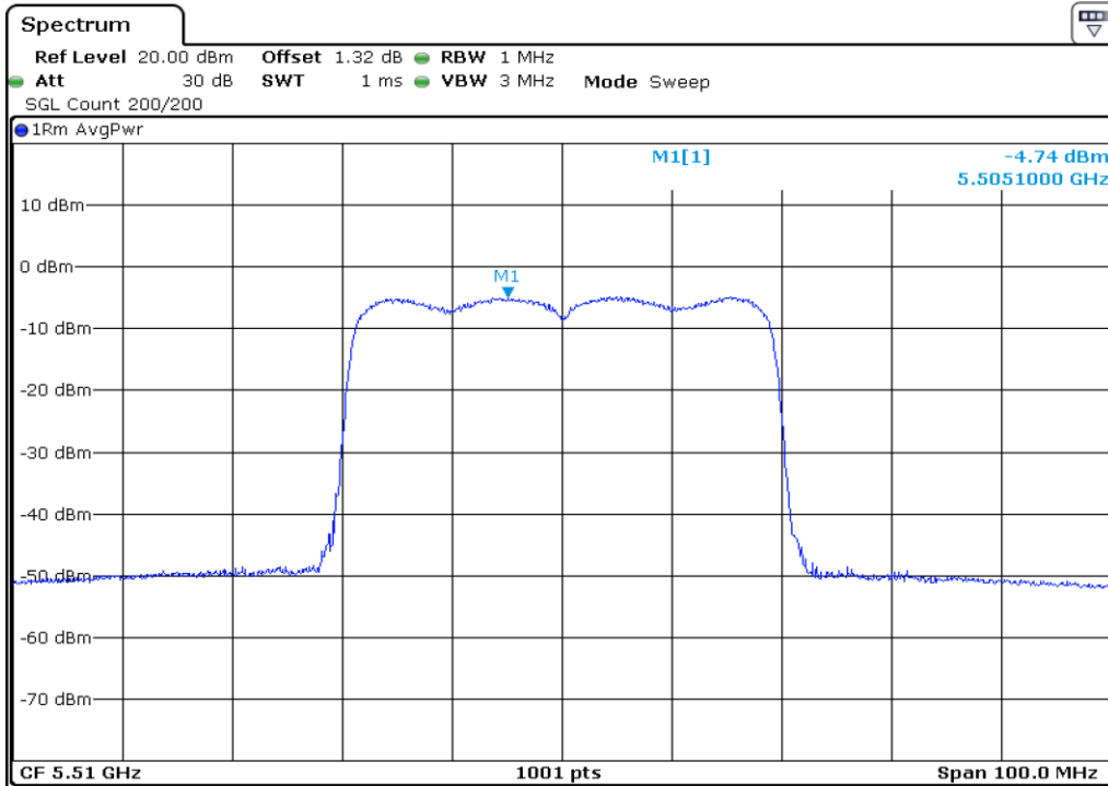
37 Peak Power Spectrul Density
