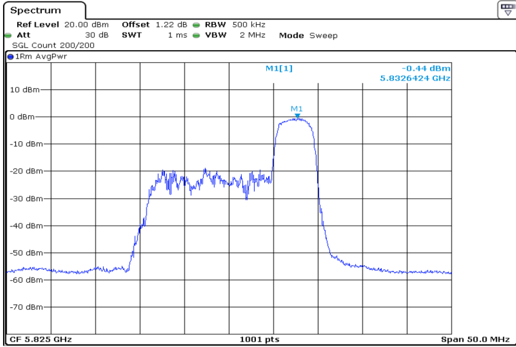
18 Peak Power Spectrual Density
