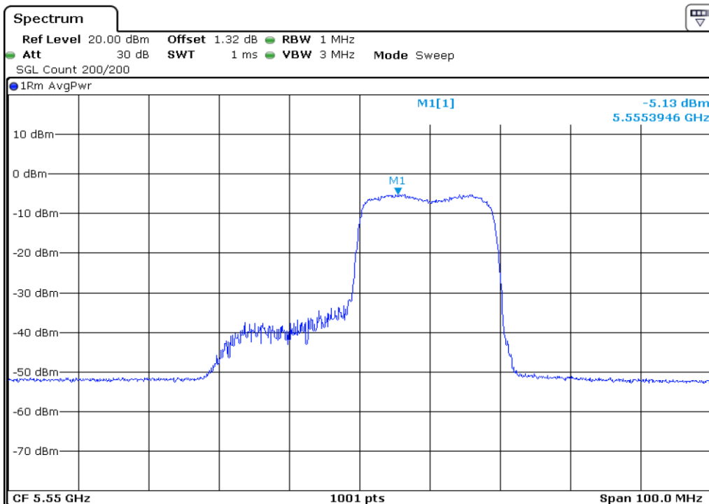
31 Peak Power Spectrul Density
