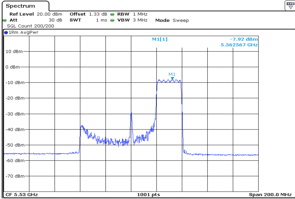
12 Peak Power Spectral Density
