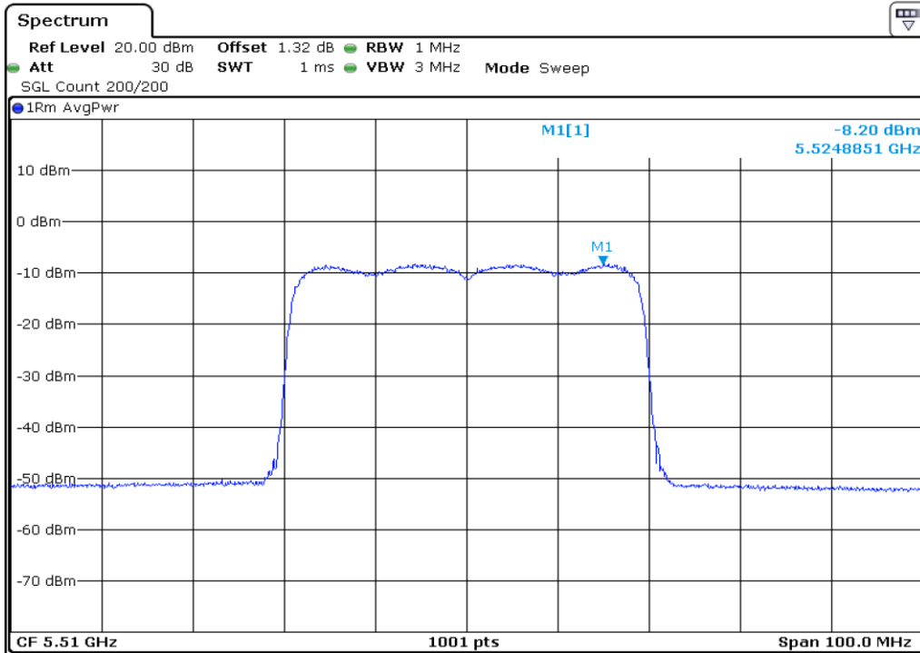
34 Peak Power Spectrul Density
