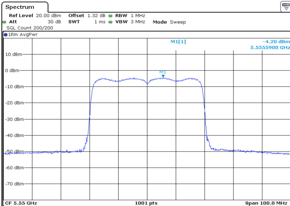
38 Peak Power Spectrul Density
