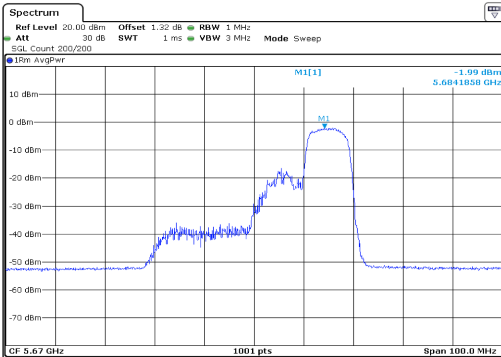
27 Peak Power Spectral Density
