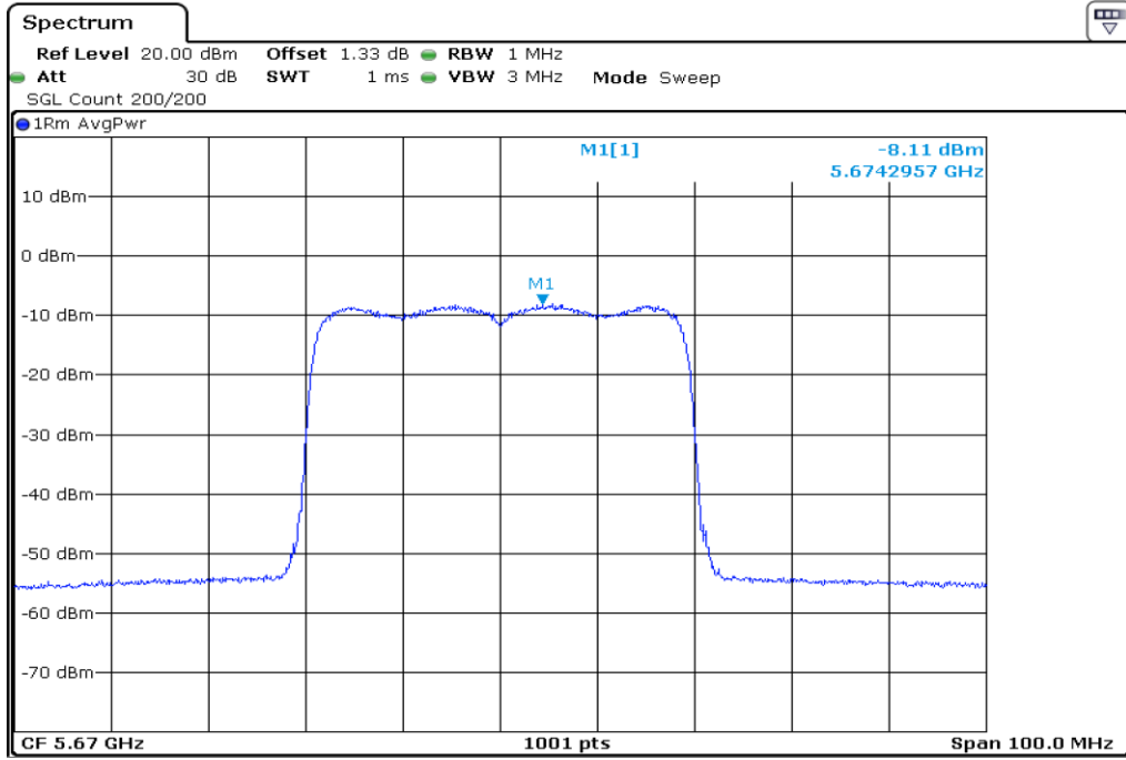
36 Peak Power Spectrul Density
