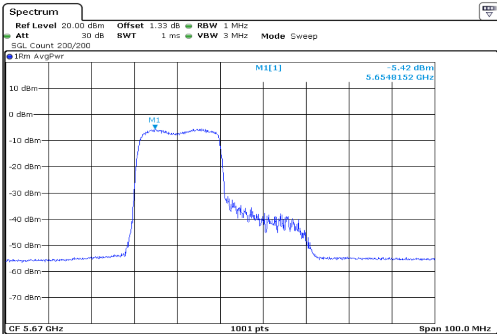
32 Peak Power Spectrul Density
