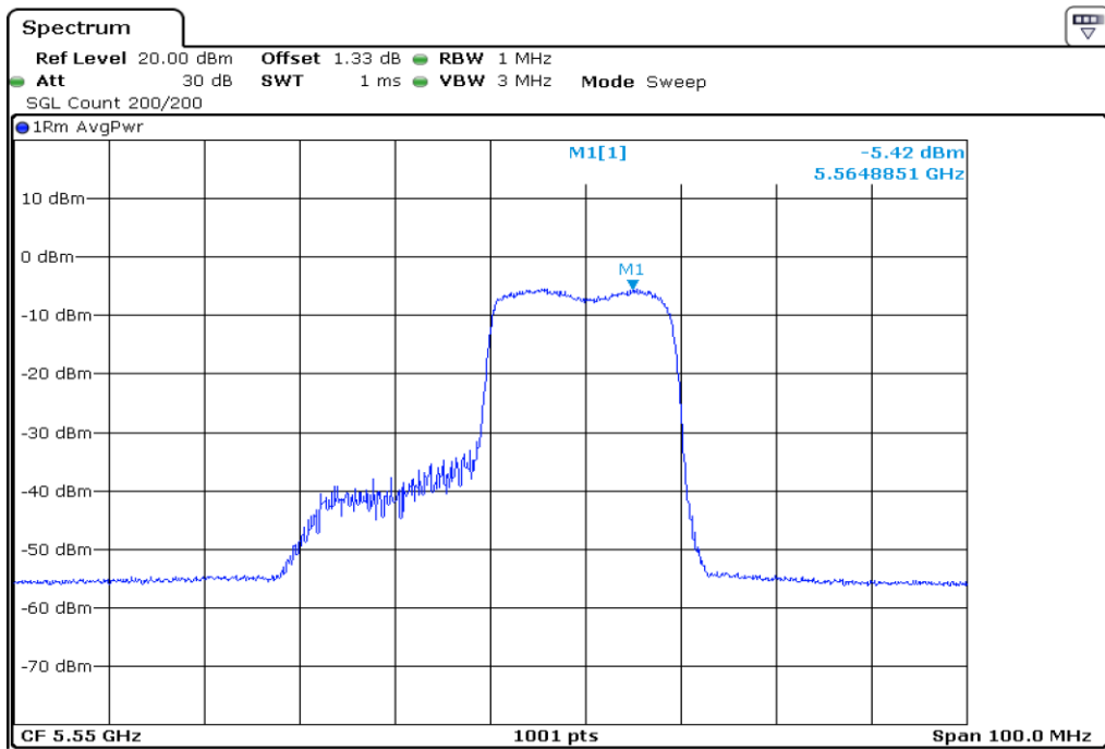
31 Peak Power Spectrul Density
