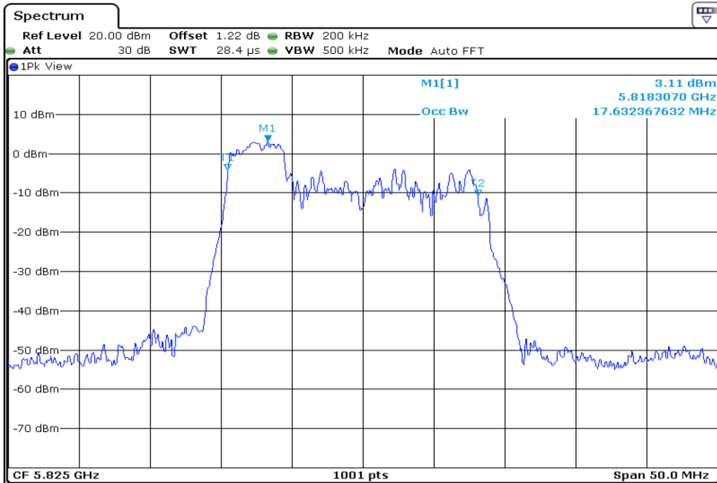
16 99% Occupied Bandwidth
