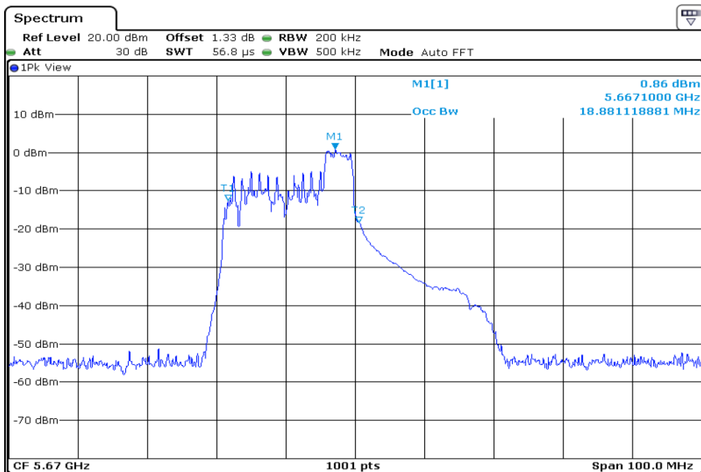
17 99% Occupied Bandwidth
