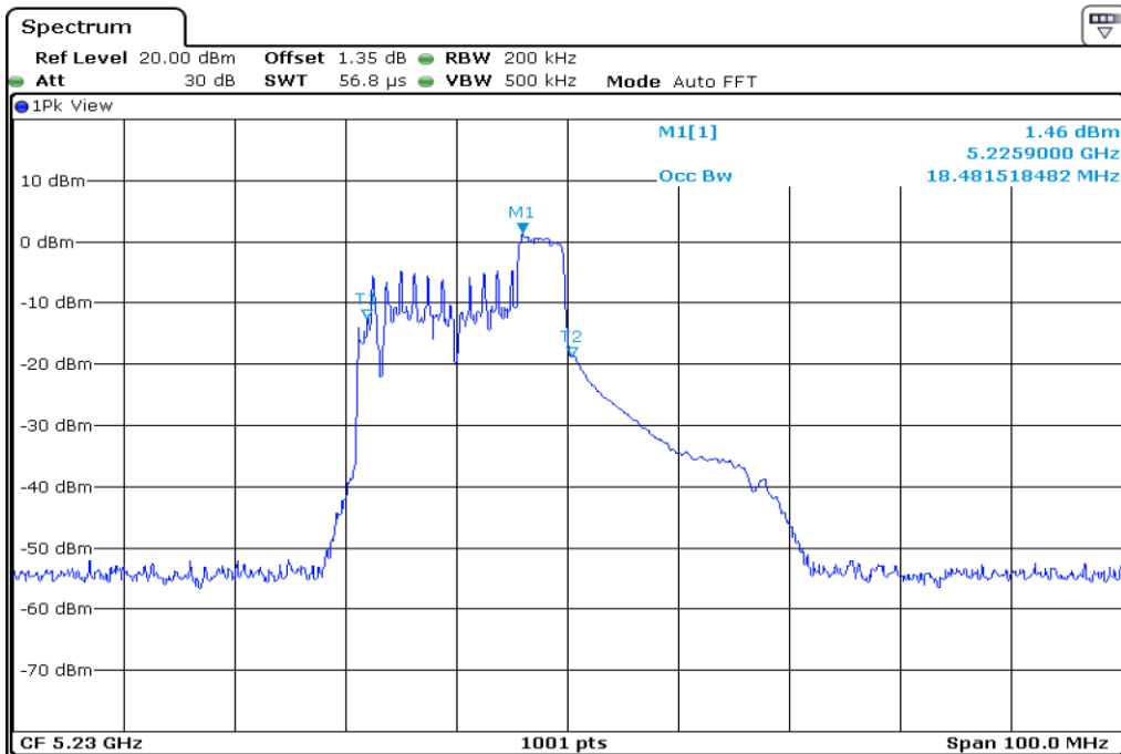
11 99% Occupied Bandwidth
