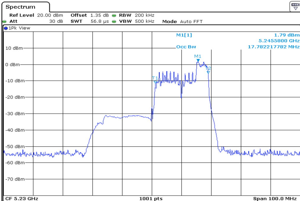
12 99% Occupied Bandwidth
