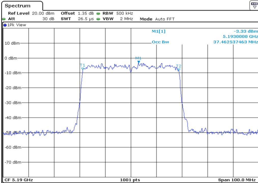
23 99% Occupied Bandwidth
