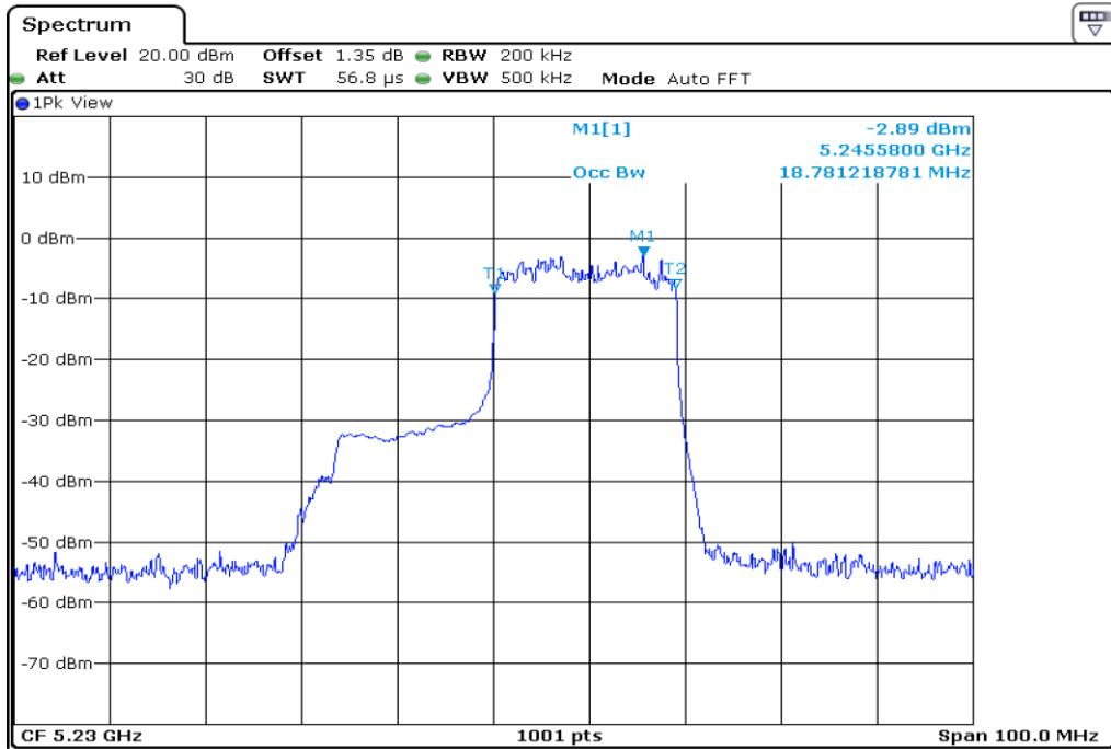
22 99% Occupied Bandwidth
