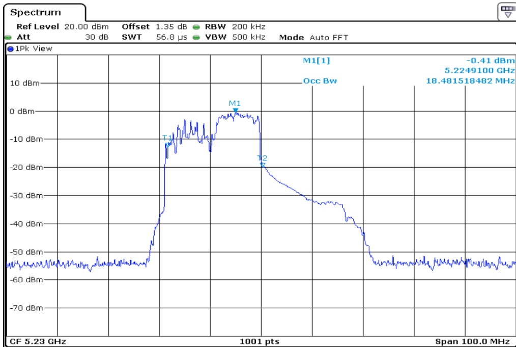
17 99% Occupied Bandwidth
