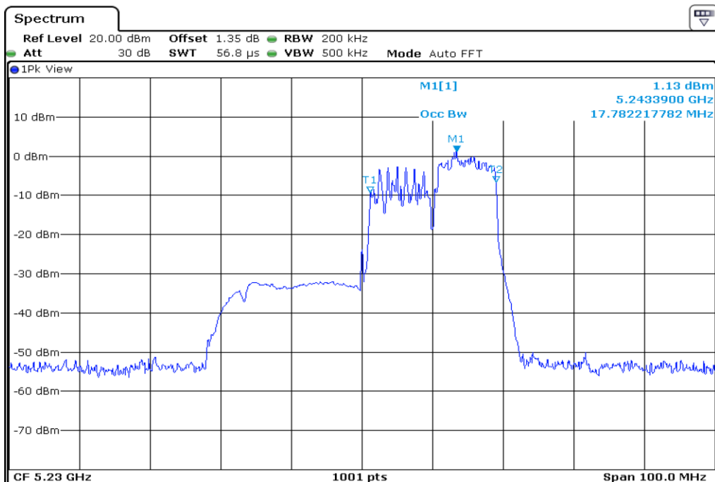
18 99% Occupied Bandwidth
