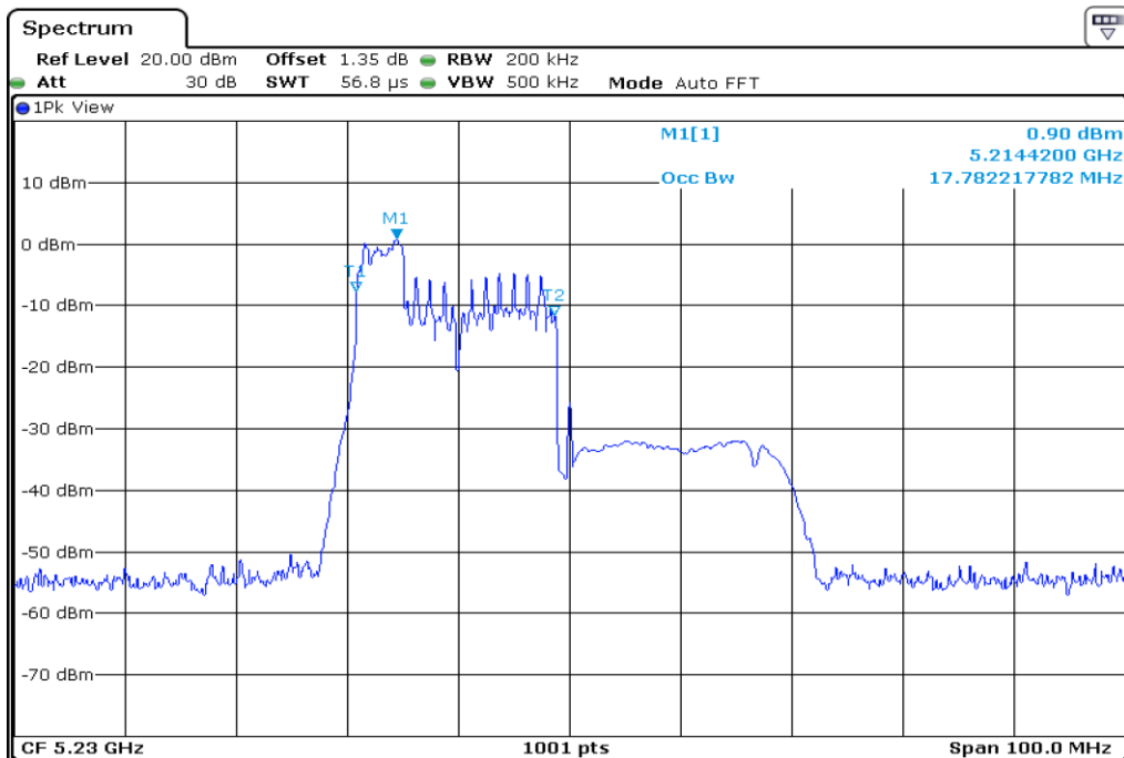
10 99% Occupied Bandwidth
