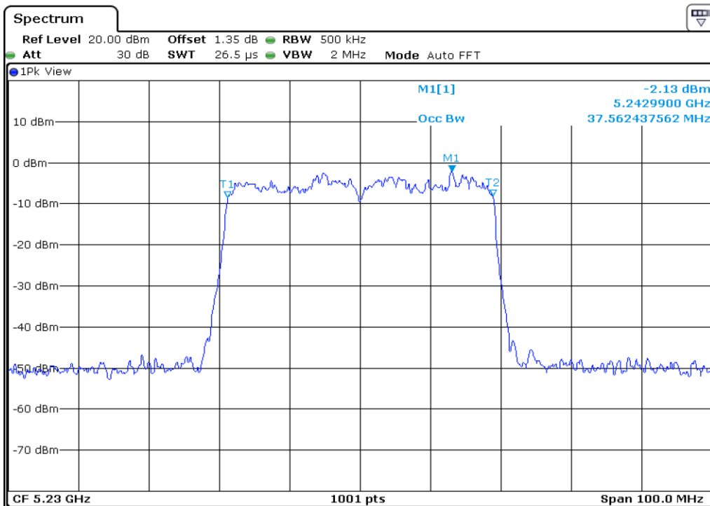
24 99% Occupied Bandwidth
