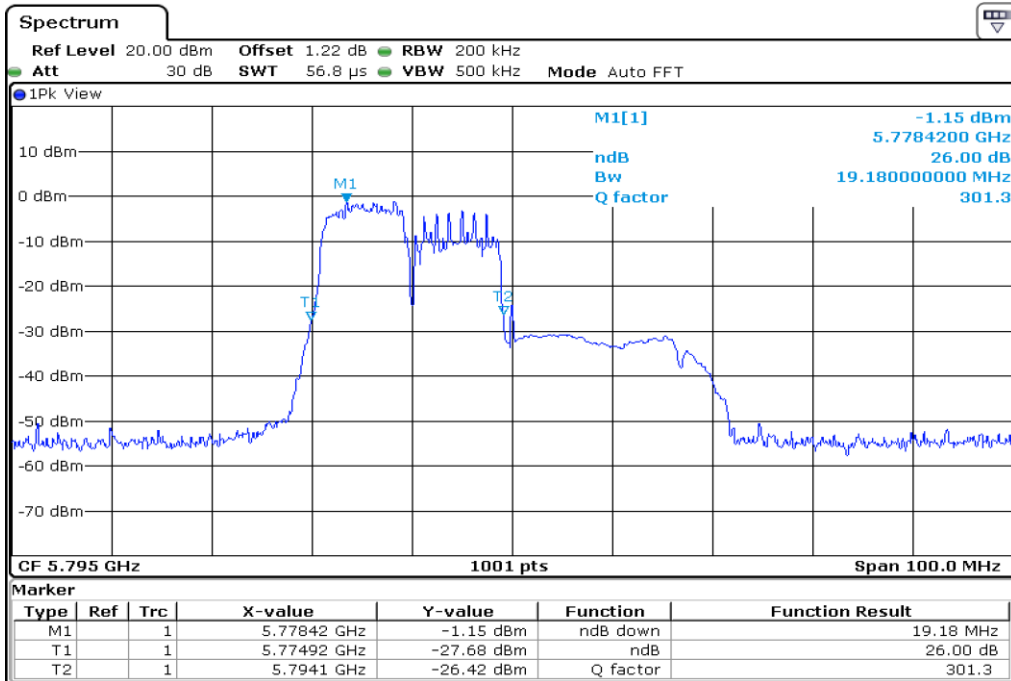
16 26 dB Bandwidth
