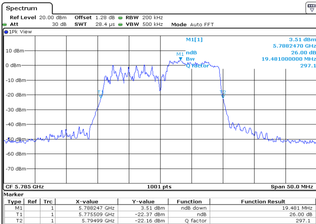
22 26 dB Bandwidth
