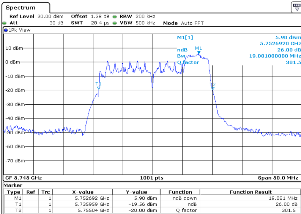
12 26 dB Bandwidth
