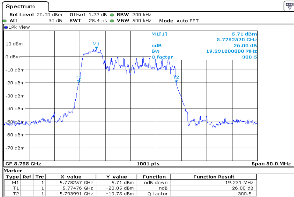
13 26 dB Bandwidth
