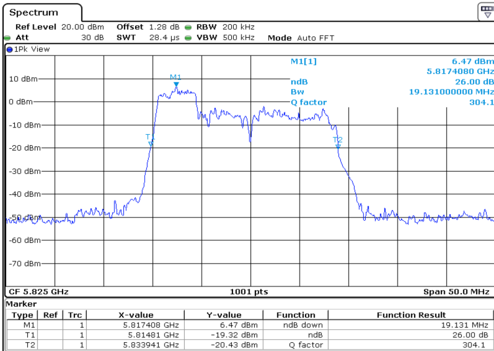
16 26 dB Bandwidth
