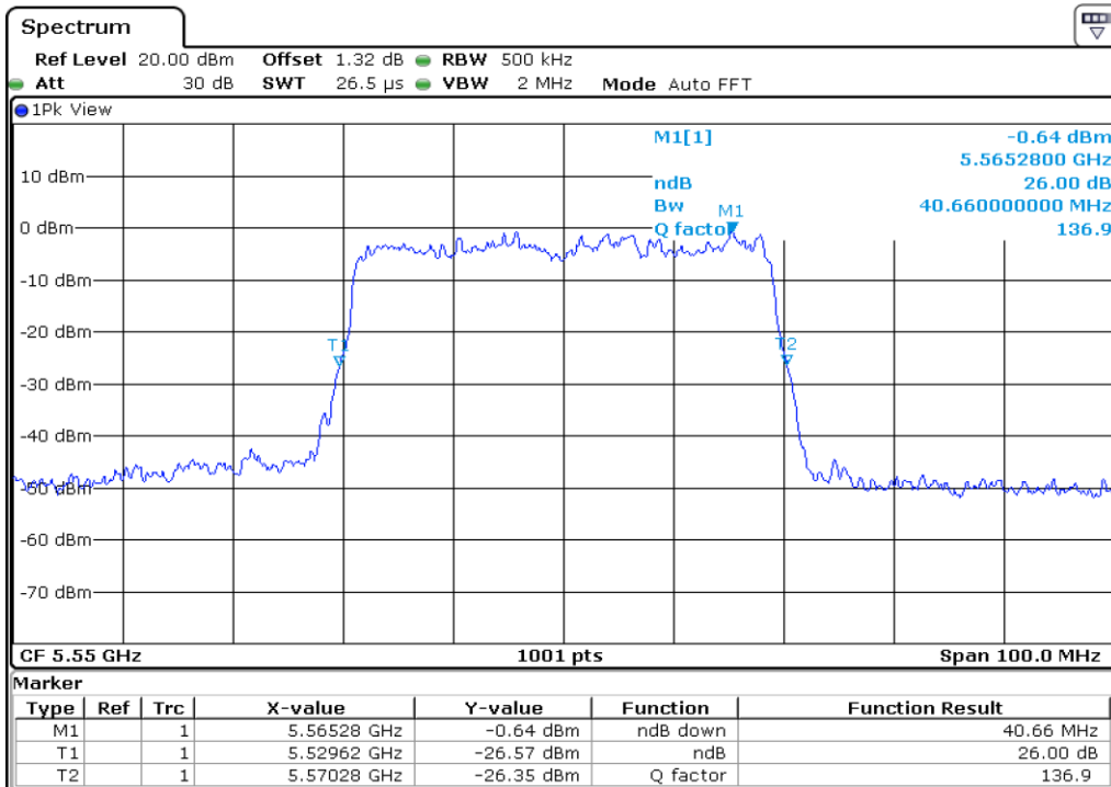
35 26 dB Bandwidth
