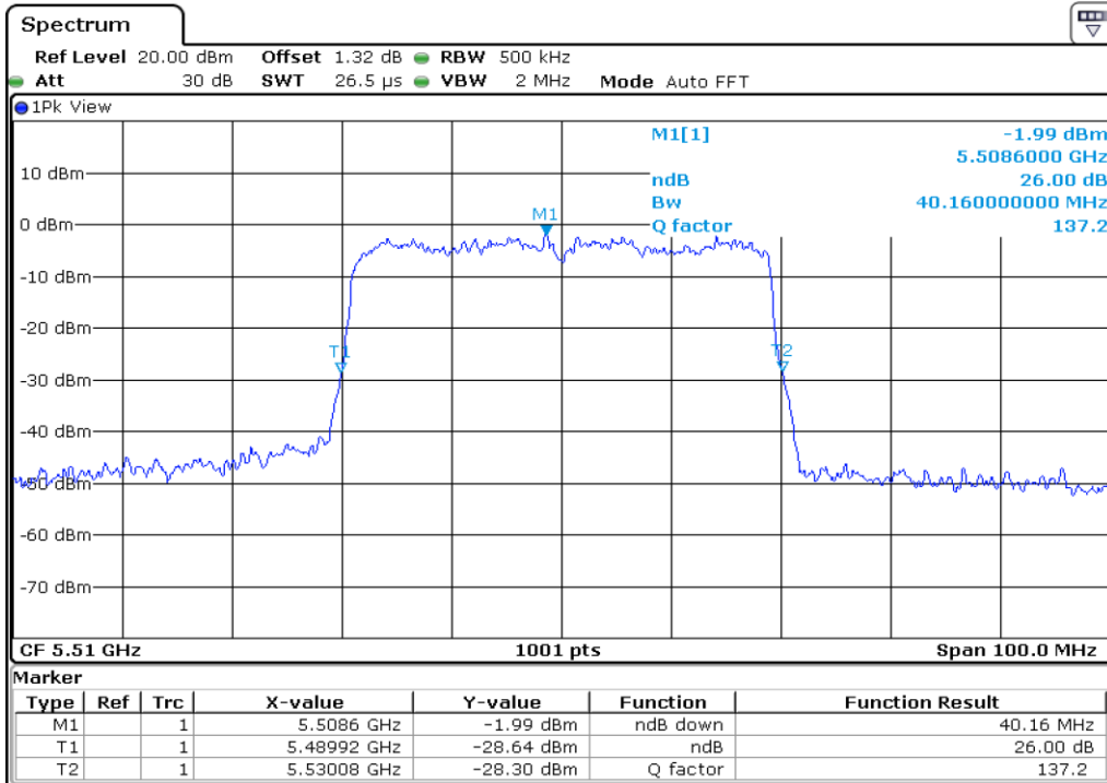
34 26 dB Bandwidth
