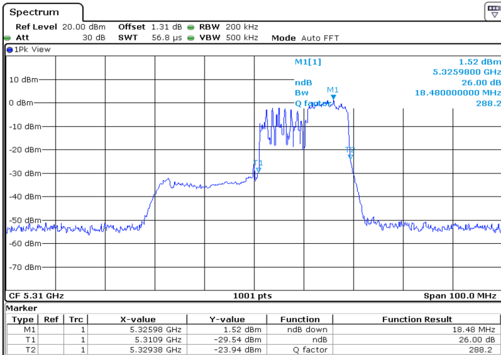
18 26 dB Bandwidth
