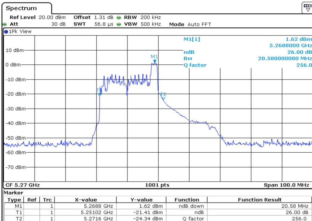
2 26 dB Bandwidth
