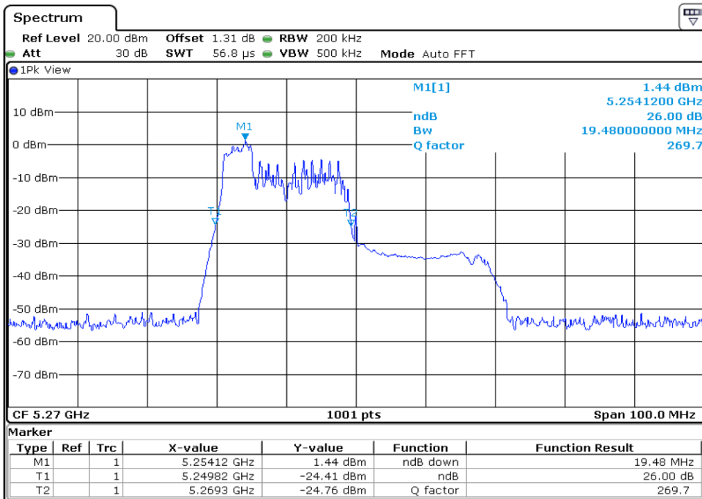
7 26 dB Bandwidth
