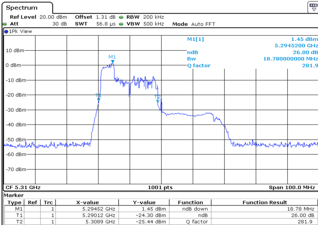
10 26 dB Bandwidth
