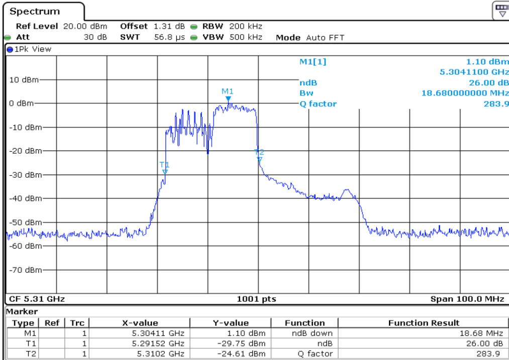
17 26 dB Bandwidth
