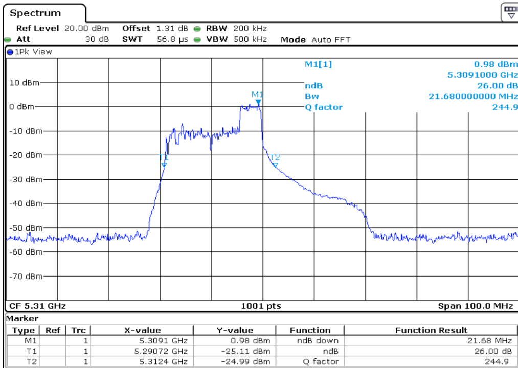
11 26 dB Bandwidth
