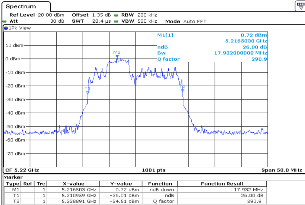
14 26 dB Bandwidth
