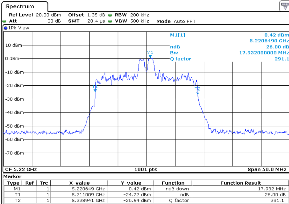
5 26 dB Bandwidth
