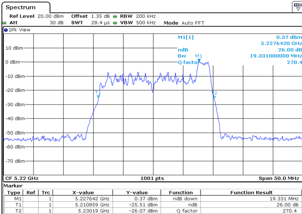
6 26 dB Bandwidth
