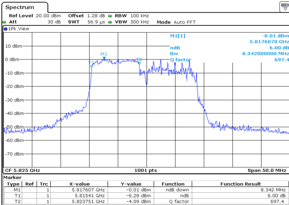
23 6 dB Bandwidth
