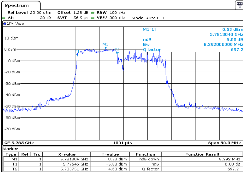
21 6 dB Bandwidth
