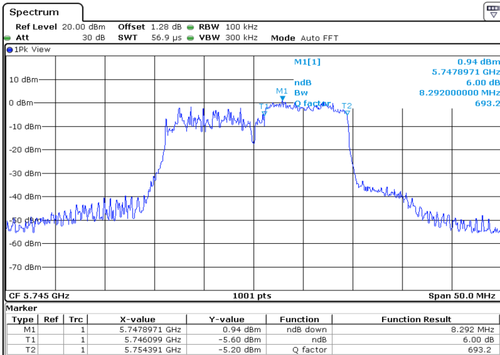
20 6 dB Bandwidth
