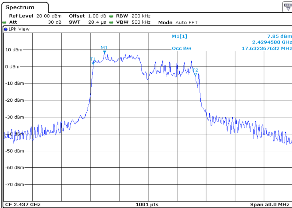
21 | 99% Occupied Bandwidth
