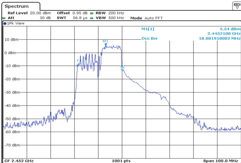
26 99% Occupied Bandwidth
