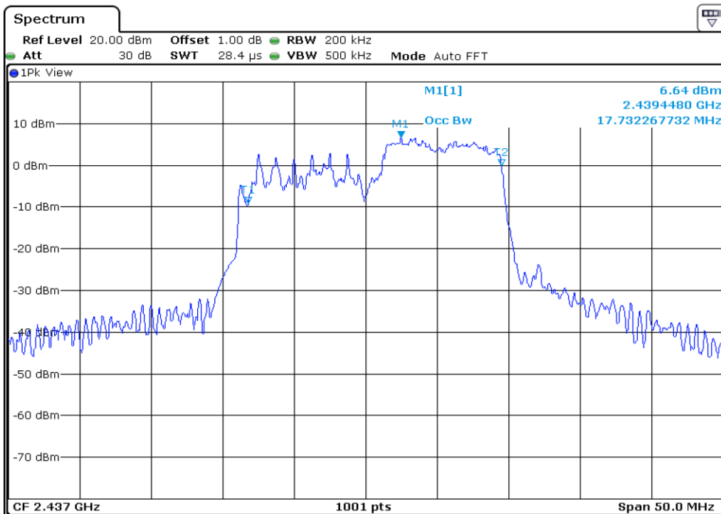
22 | 99% Occupied Bandwidth
