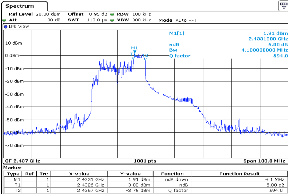
14 6 dB Bandwidth
