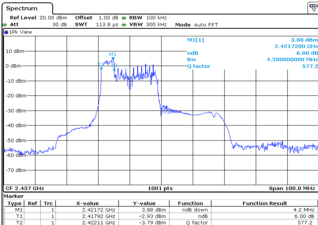
13 6 dB Bandwidth
