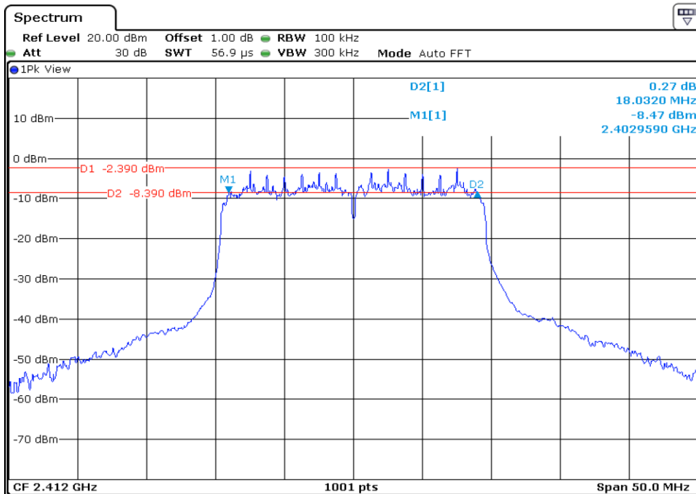
28 6 dB Bandwidth
