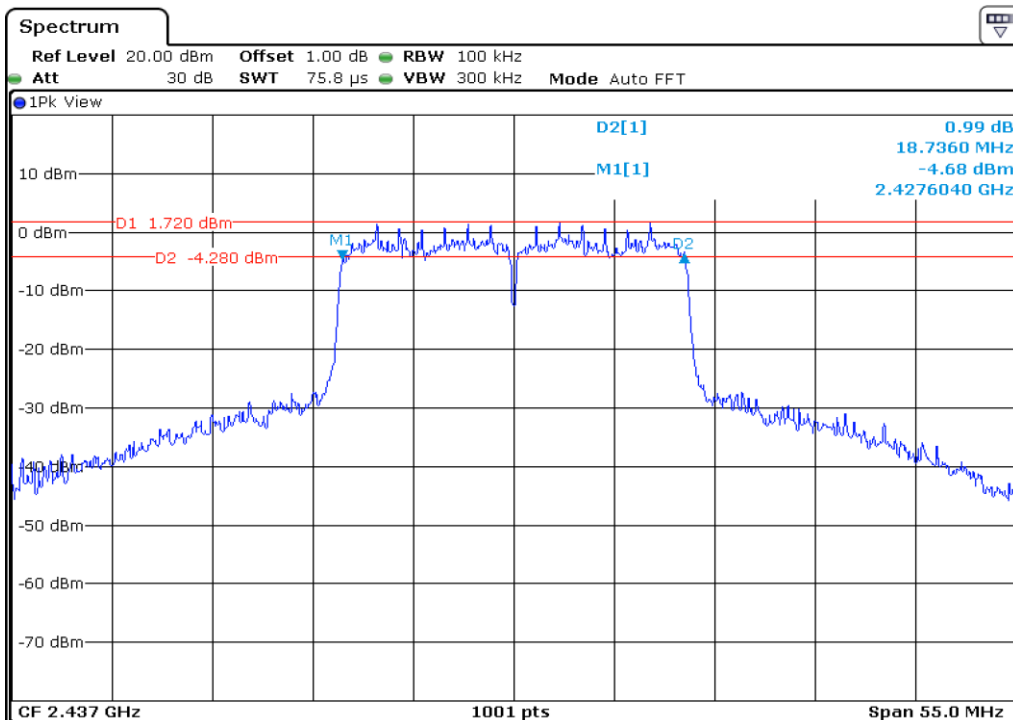
26 6 dB Bandwidth
