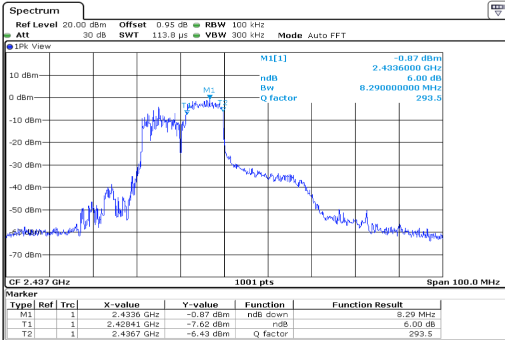
23 6 dB Bandwidth
