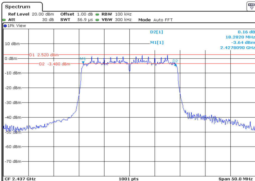
29 6 dB Bandwidth
