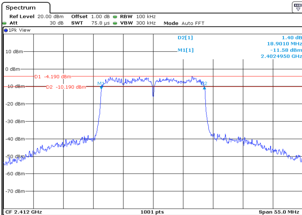
25 6 dB Bandwidth
