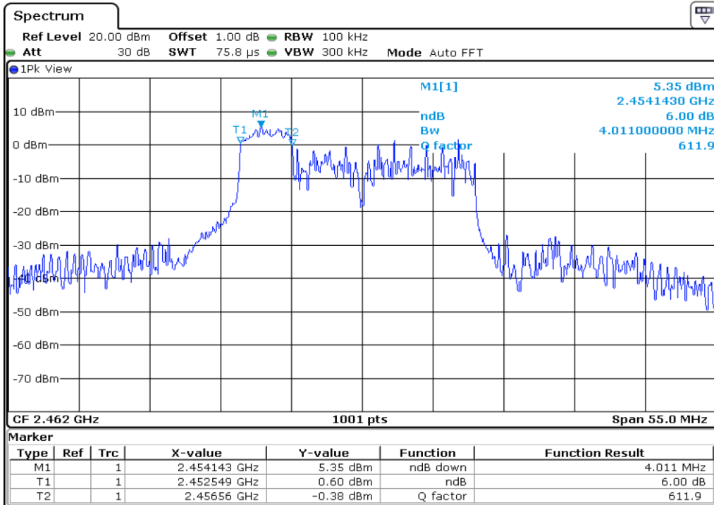
16 6 dB Bandwidth
