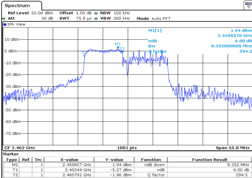
23 6 dB Bandwidth
