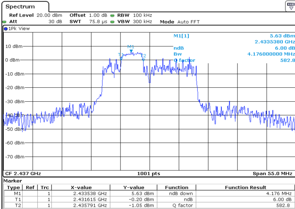
14 6 dB Bandwidth
