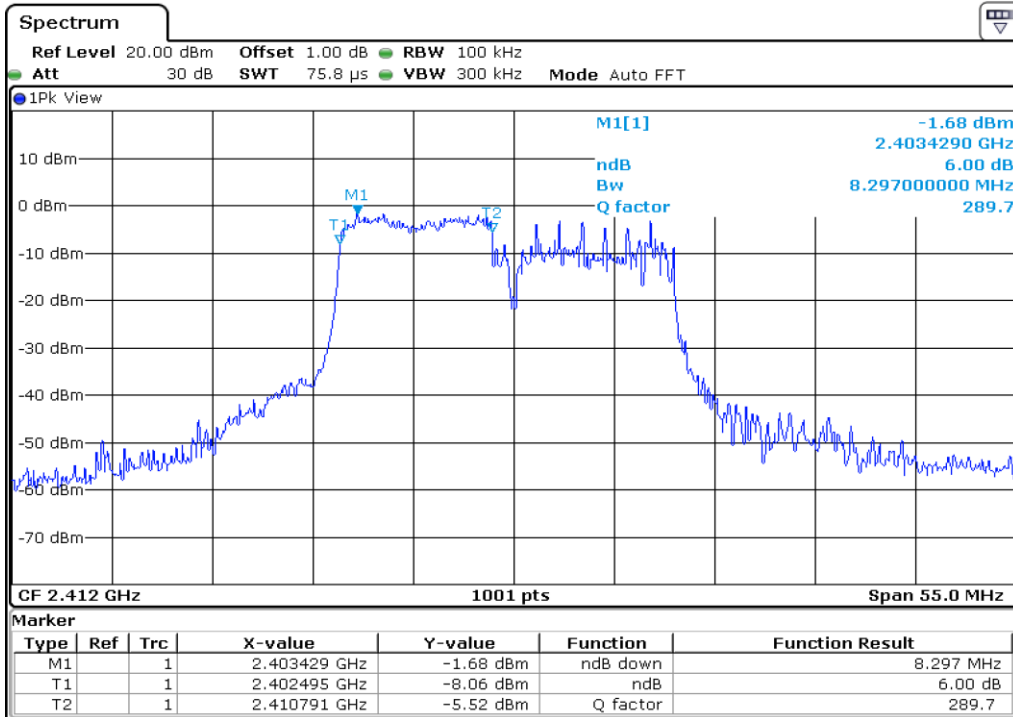
19 6 dB Bandwidth
