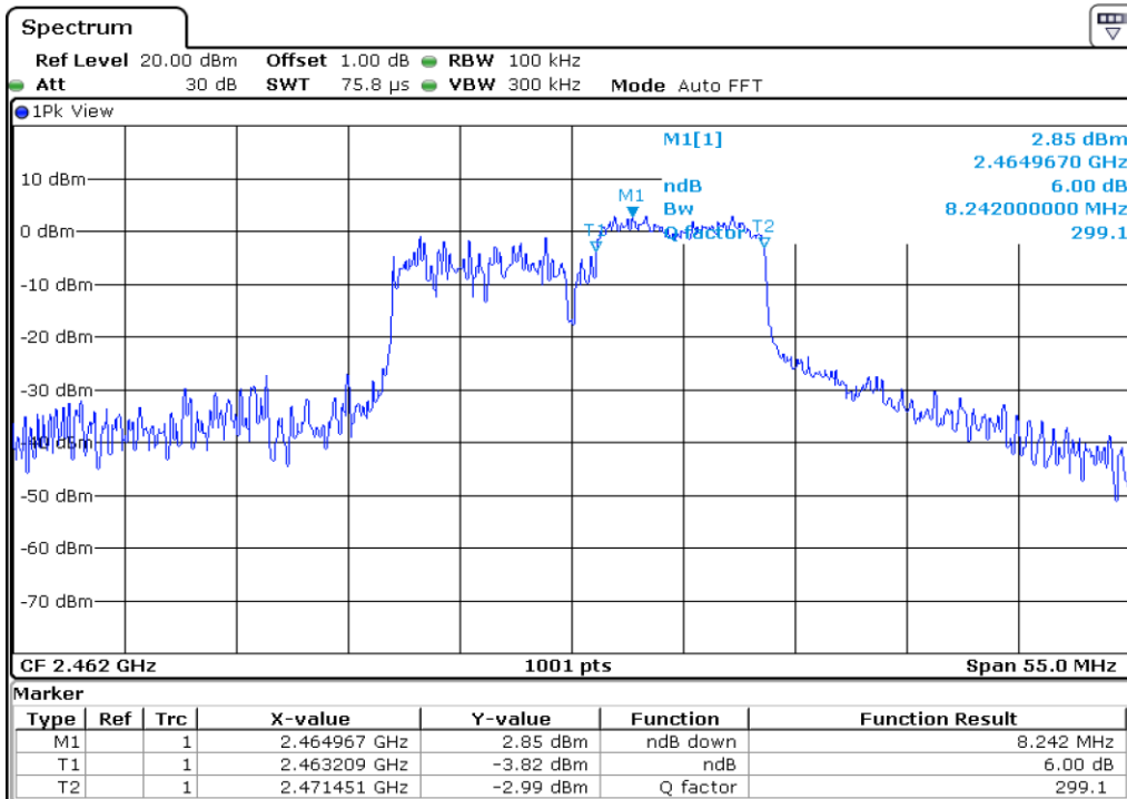
24 6 dB Bandwidth
