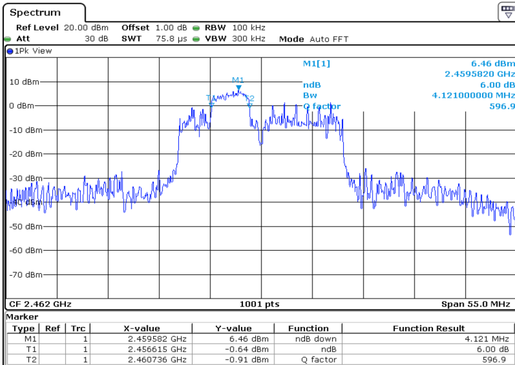
17 6 dB Bandwidth
