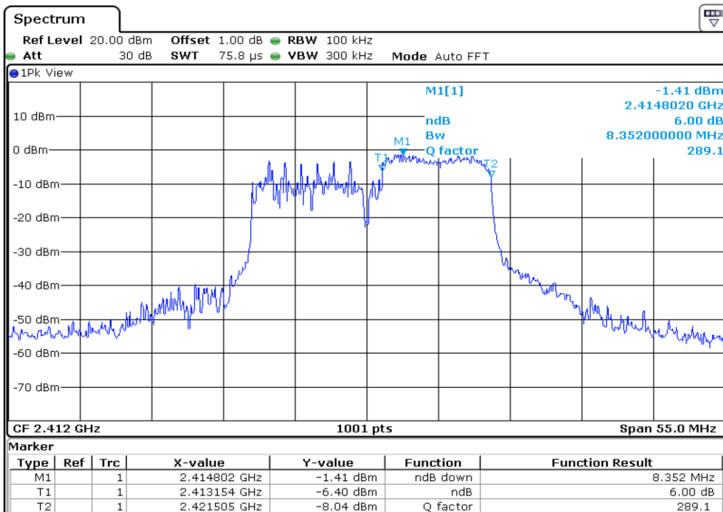
20 6 dB Bandwidth
