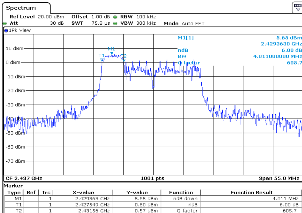
13 6 dB Bandwidth
