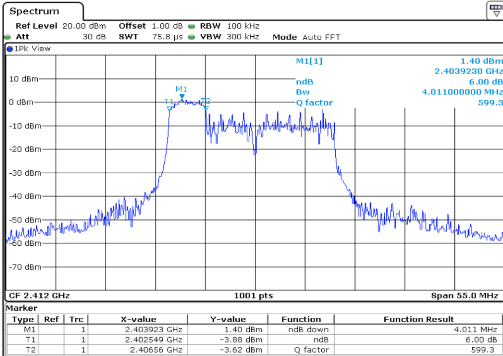
10 6 dB Bandwidth
