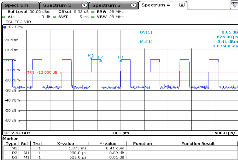
2 Duty Cycle
