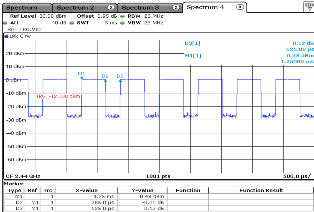
1 Duty Cycle
