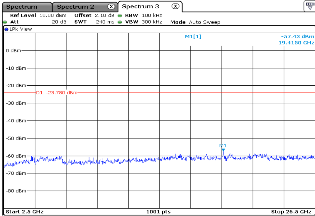
9.2 | 100 kHz Bandwidth Outside The Frequency Band
