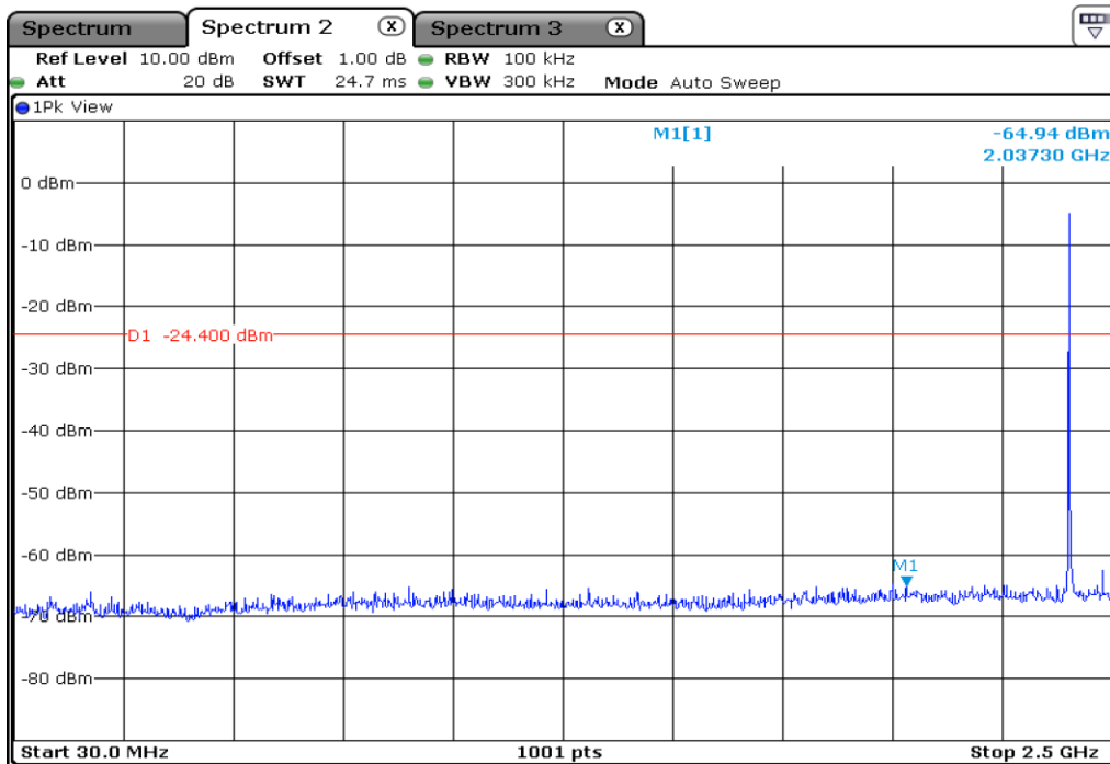
7.1 | 100 kHz Bandwidth Outside The Frequency Band
