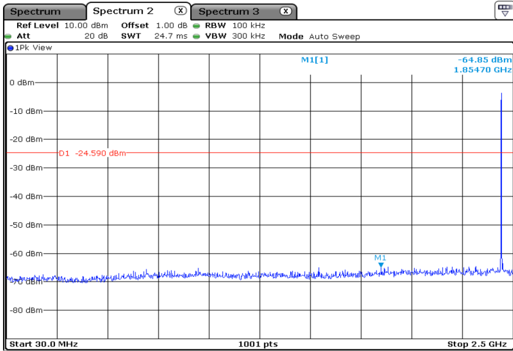
5.1 100 kHz Bandwidth Outside The Frequency Band
