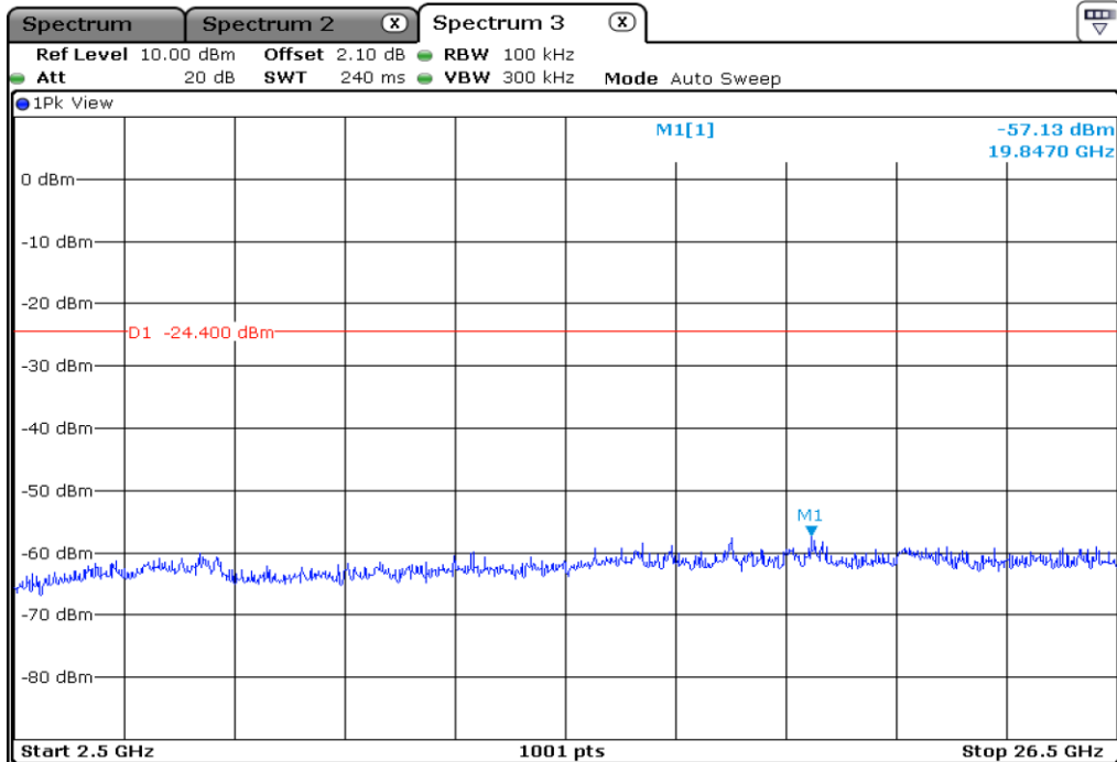
7.2 100 kHz Bandwidth Outside The Frequency Band
