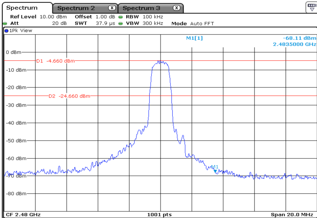
6 | 100 kHz Bandwidth Outside The Frequency Band
