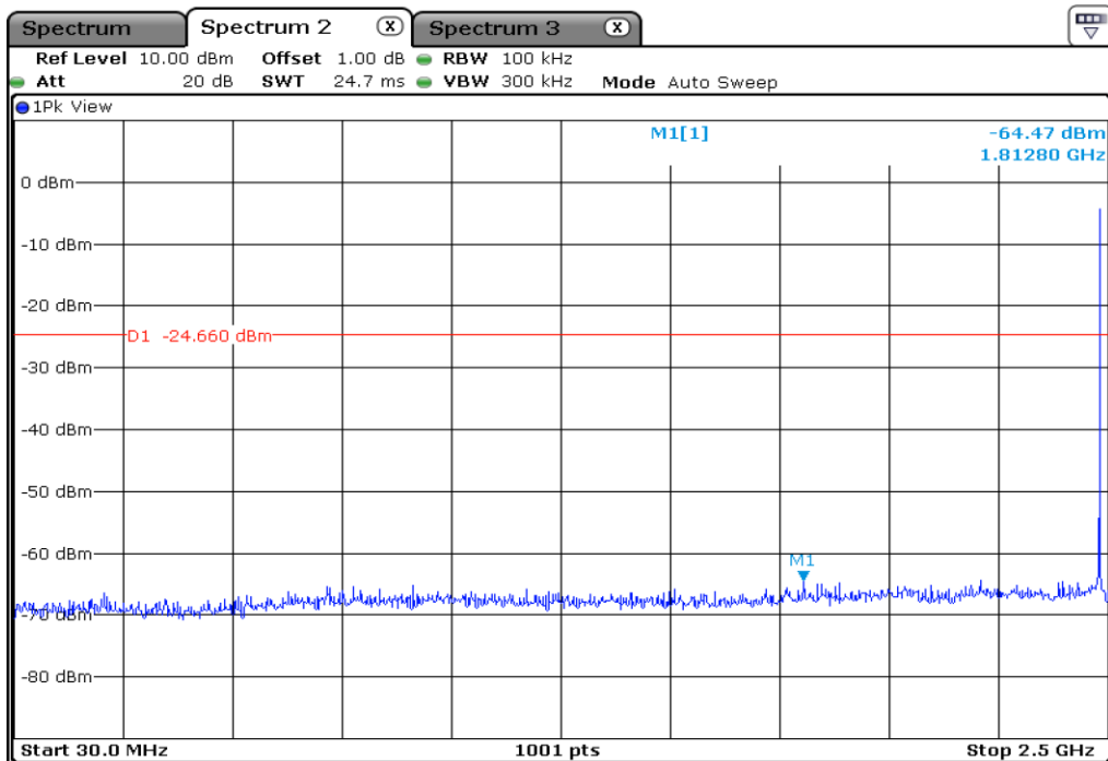
6.1 | 100 kHz Bandwidth Outside The Frequency Band
