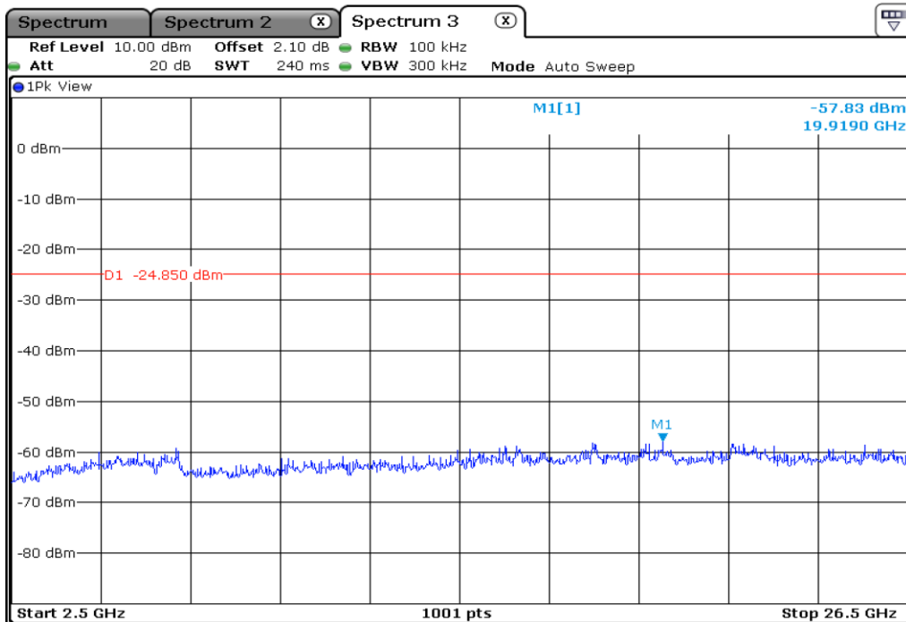
8.2 100 kHz Bandwidth Outside The Frequency Band
