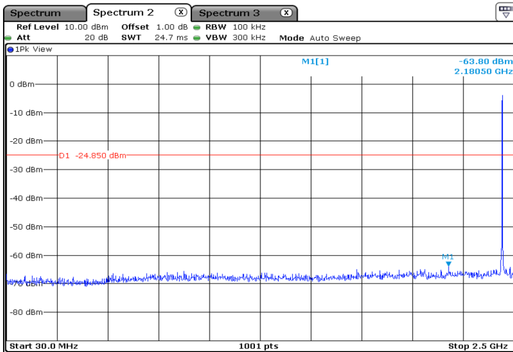
8.1 100 kHz Bandwidth Outside The Frequency Band
