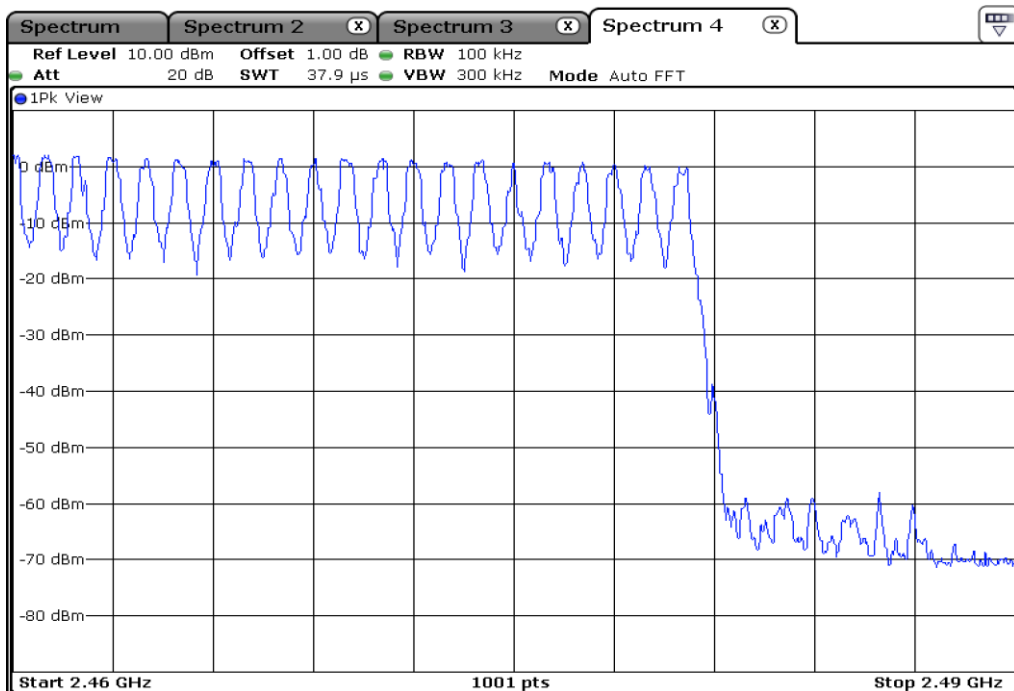
4 Number Of Hopping Channels
