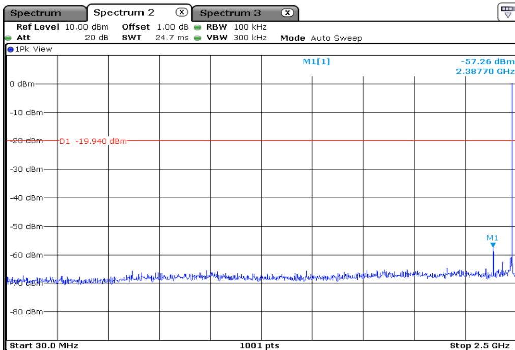
3.1 100 kHz Bandwidth Outside The Frequency Band
