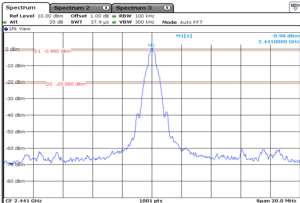
2 100 kHz Bandwidth Outside The Frequency Band
