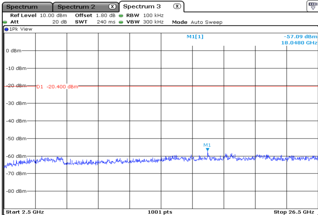
1.2 100 kHz Bandwidth Outside The Frequency Band
