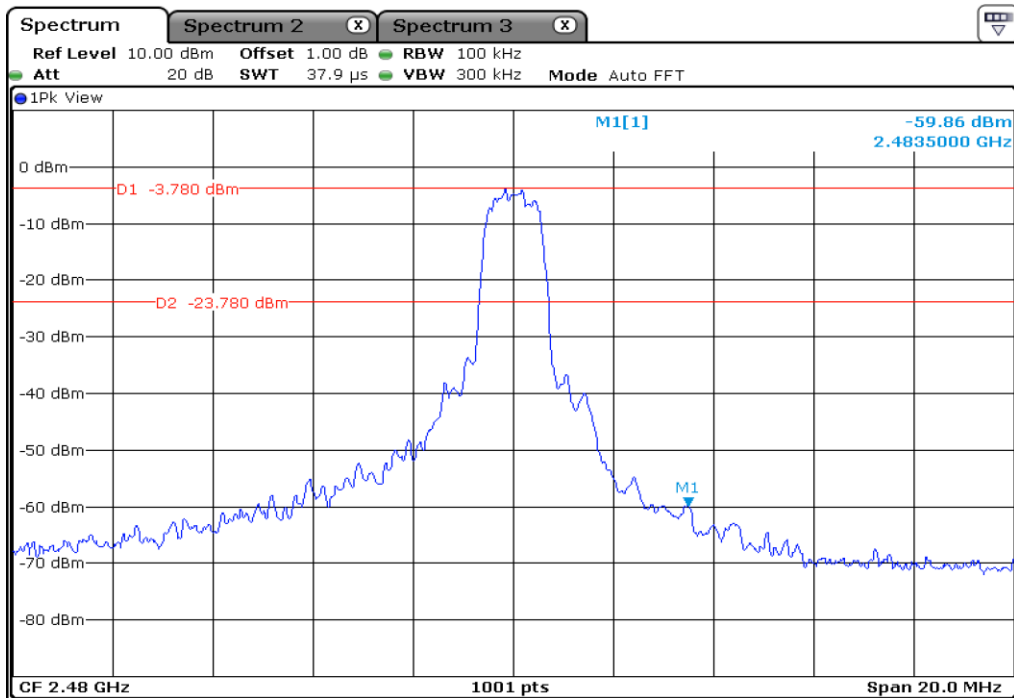
9 | 100 kHz Bandwidth Outside The Frequency Band
