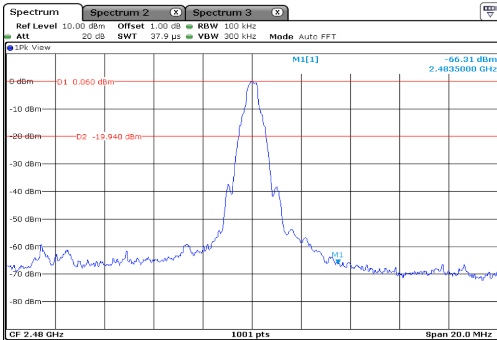
3 100 kHz Bandwidth Outside The Frequency Band
