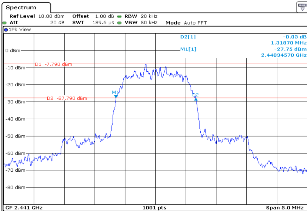
5 Minimum 20 dB Bandwidth
