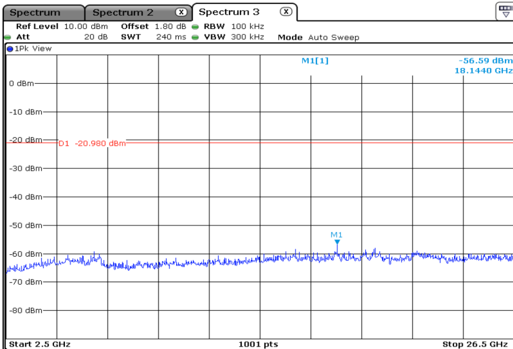
2.2 100 kHz Bandwidth Outside The Frequency Band
