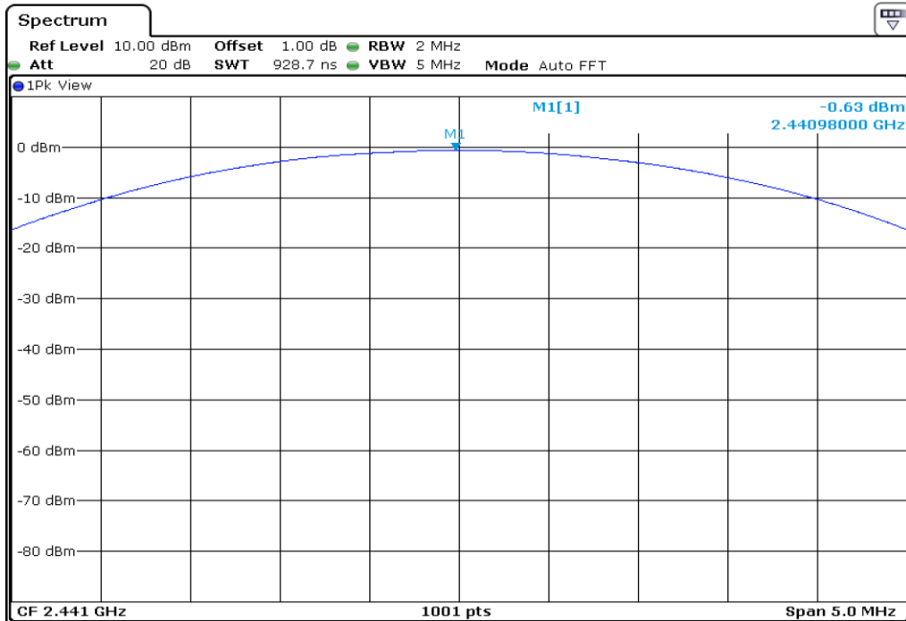
8 Maimum Peak Output Power
