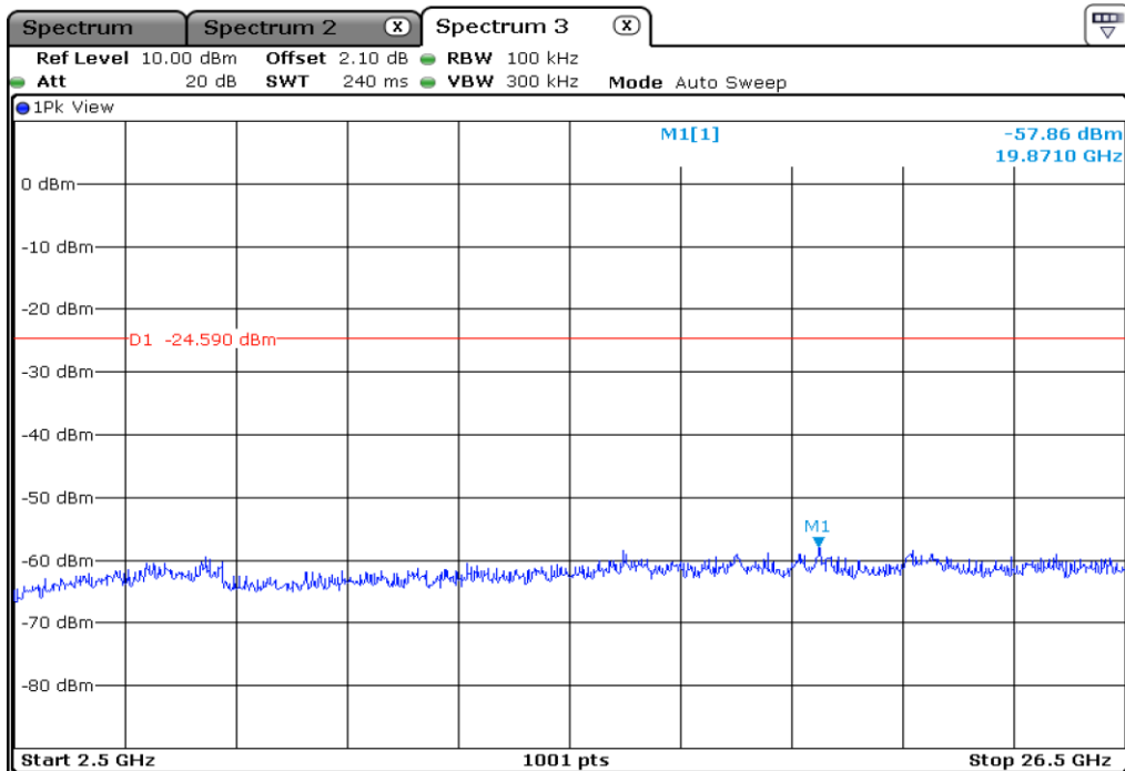
5.2 100 kHz Bandwidth Outside The Frequency Band
