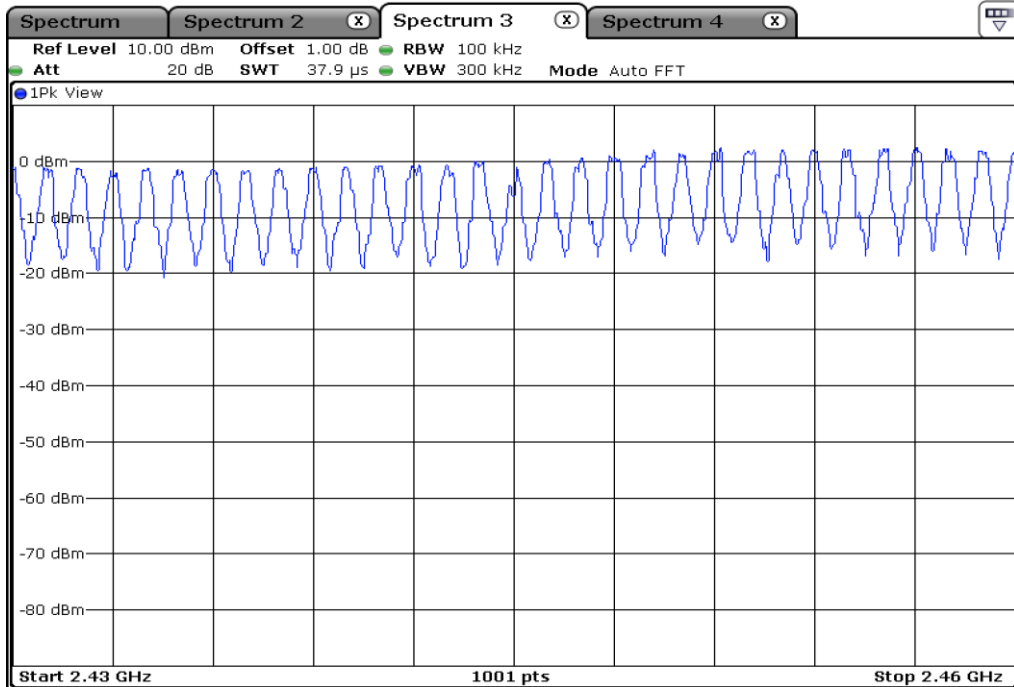
3 Number Of Hopping Channels
