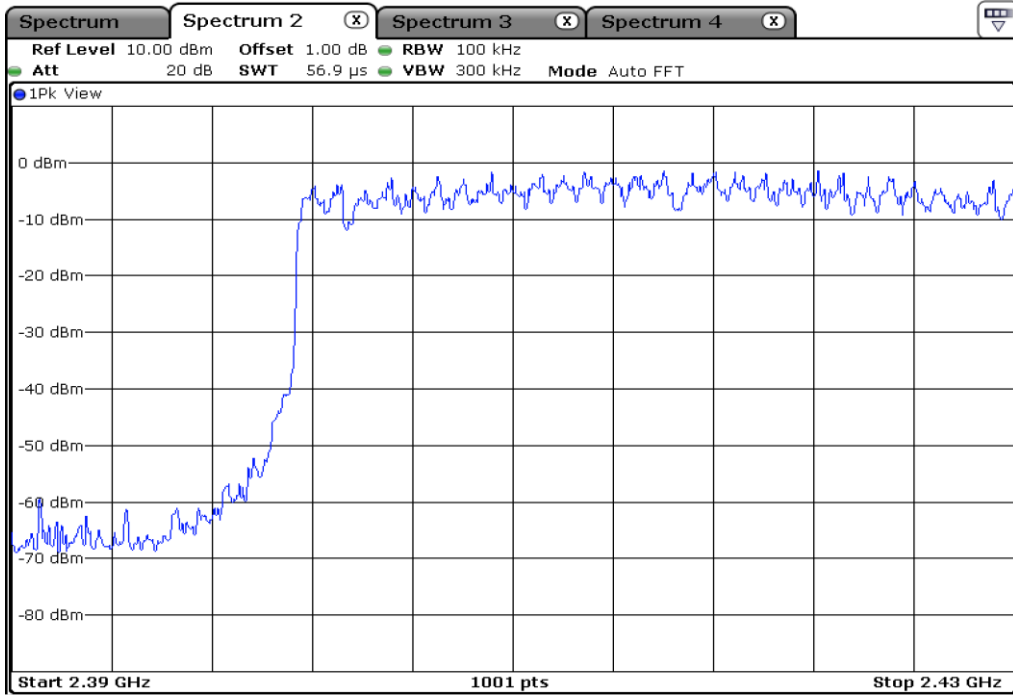
10 Number Of Hopping Channels
