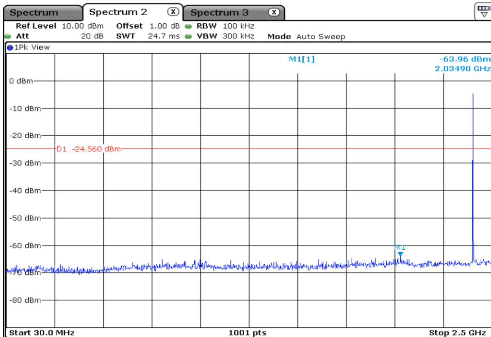
4.1 | 100 kHz Bandwidth Outside The Frequency Band
