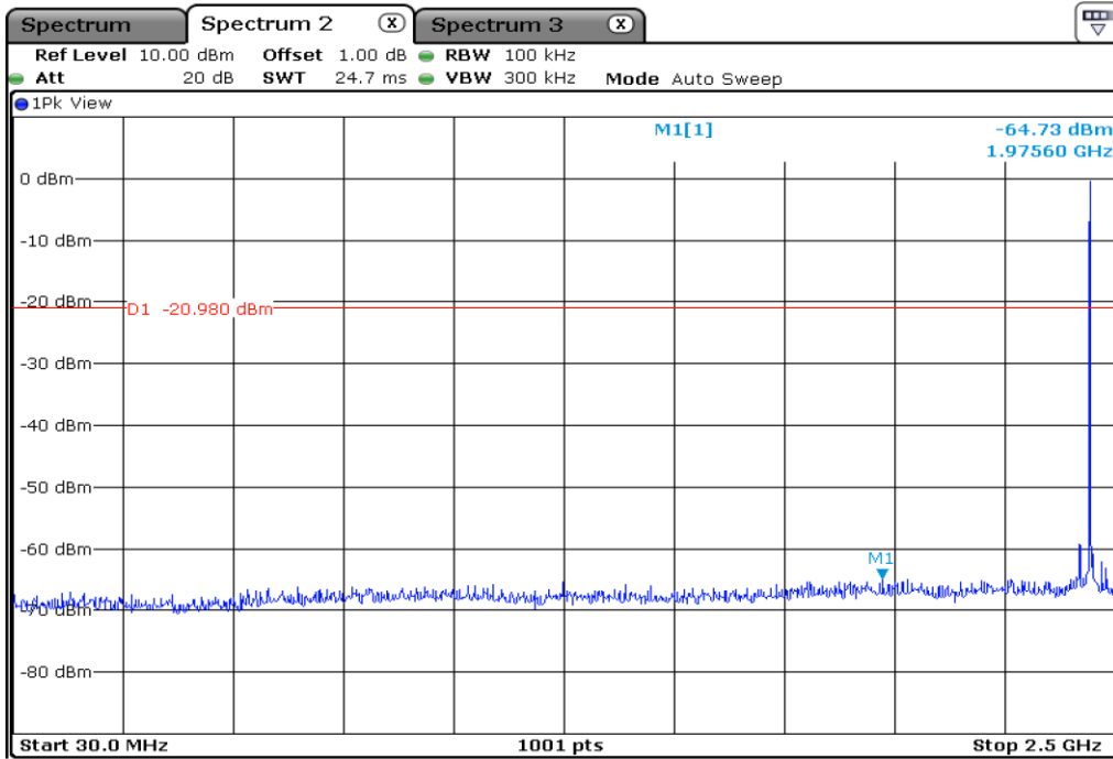
2.1 100 kHz Bandwidth Outside The Frequency Band
