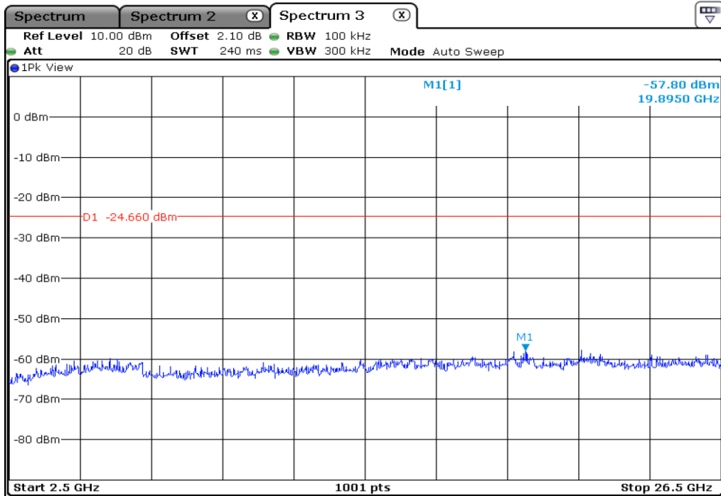
6.2 100 kHz Bandwidth Outside The Frequency Band
