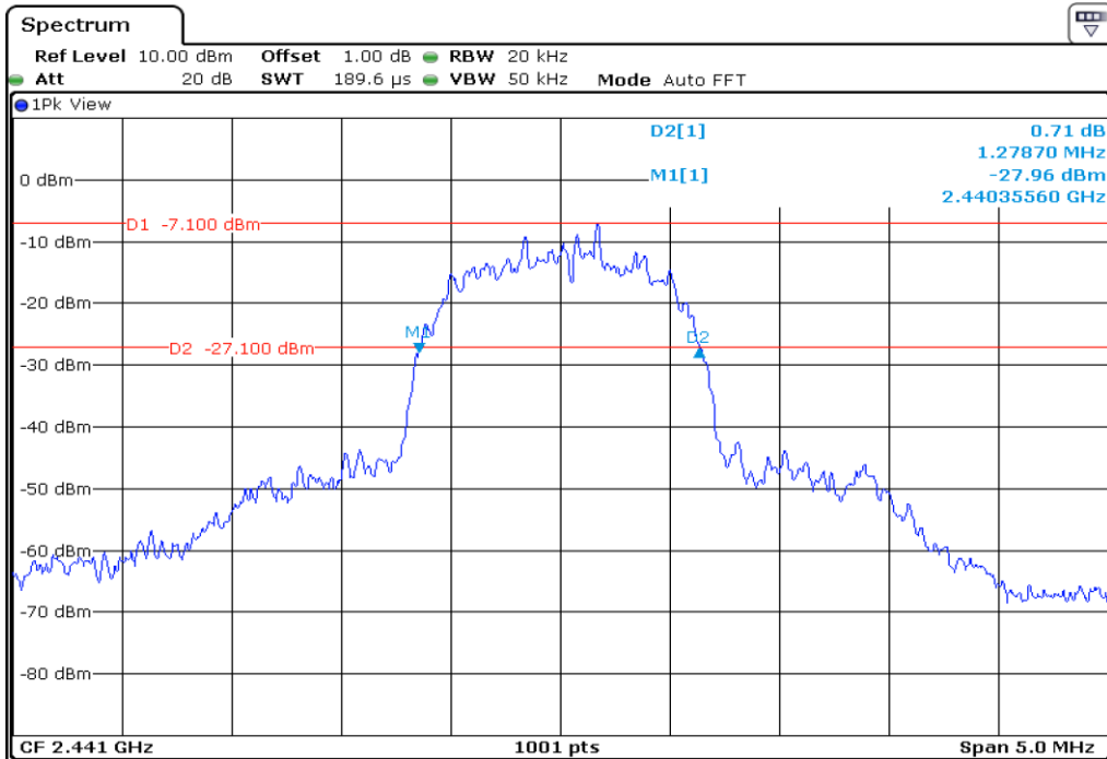
8 Minimum 20 dB Bandwidth
